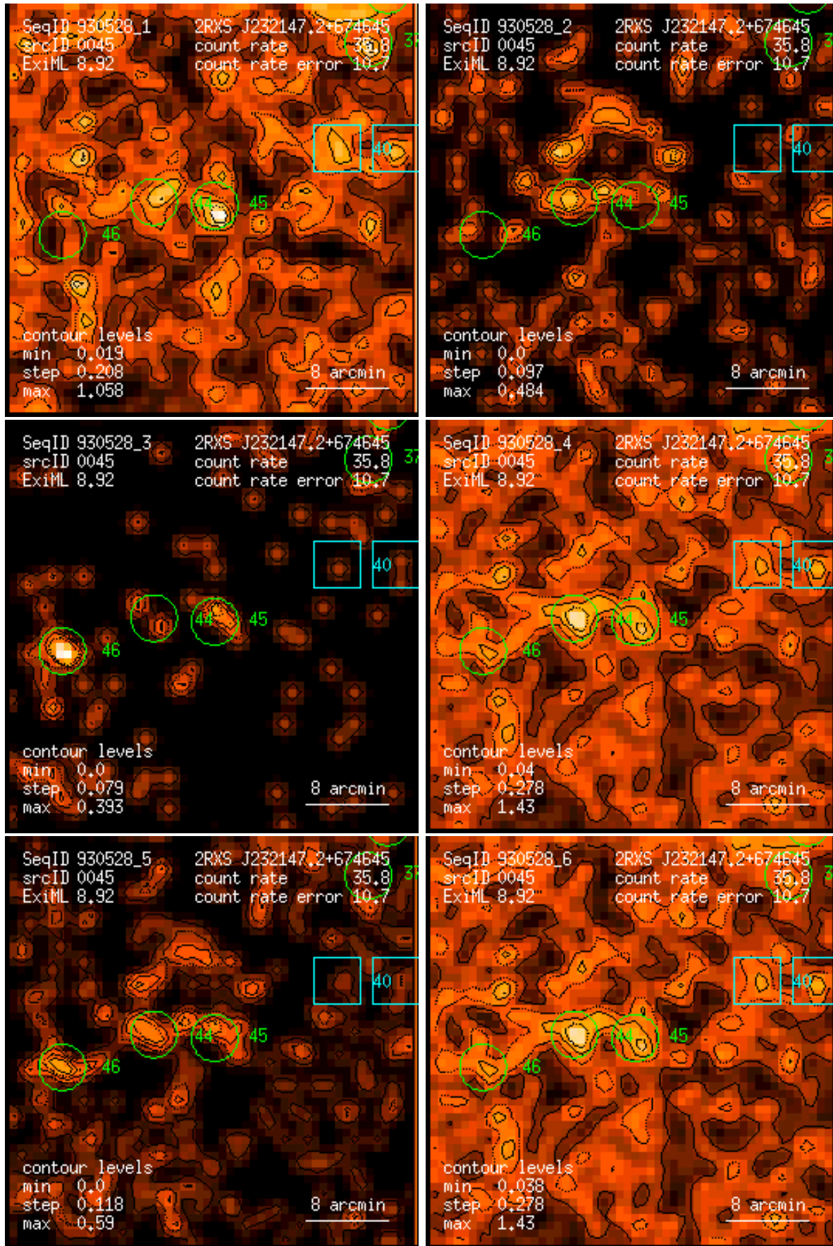
Figure 45: RASS 930528: detection 0045: band rate images, Gaussian filter: (1) PSPC channels 11 – 41, (2) 52 – 90, (3) 91 – 201, (4) 11 – 235, (5) 52 – 201, (6) 11 – 201. Broad band rates in counts/ks. Band rate contour levels in counts/ks/arcmin 2 .
