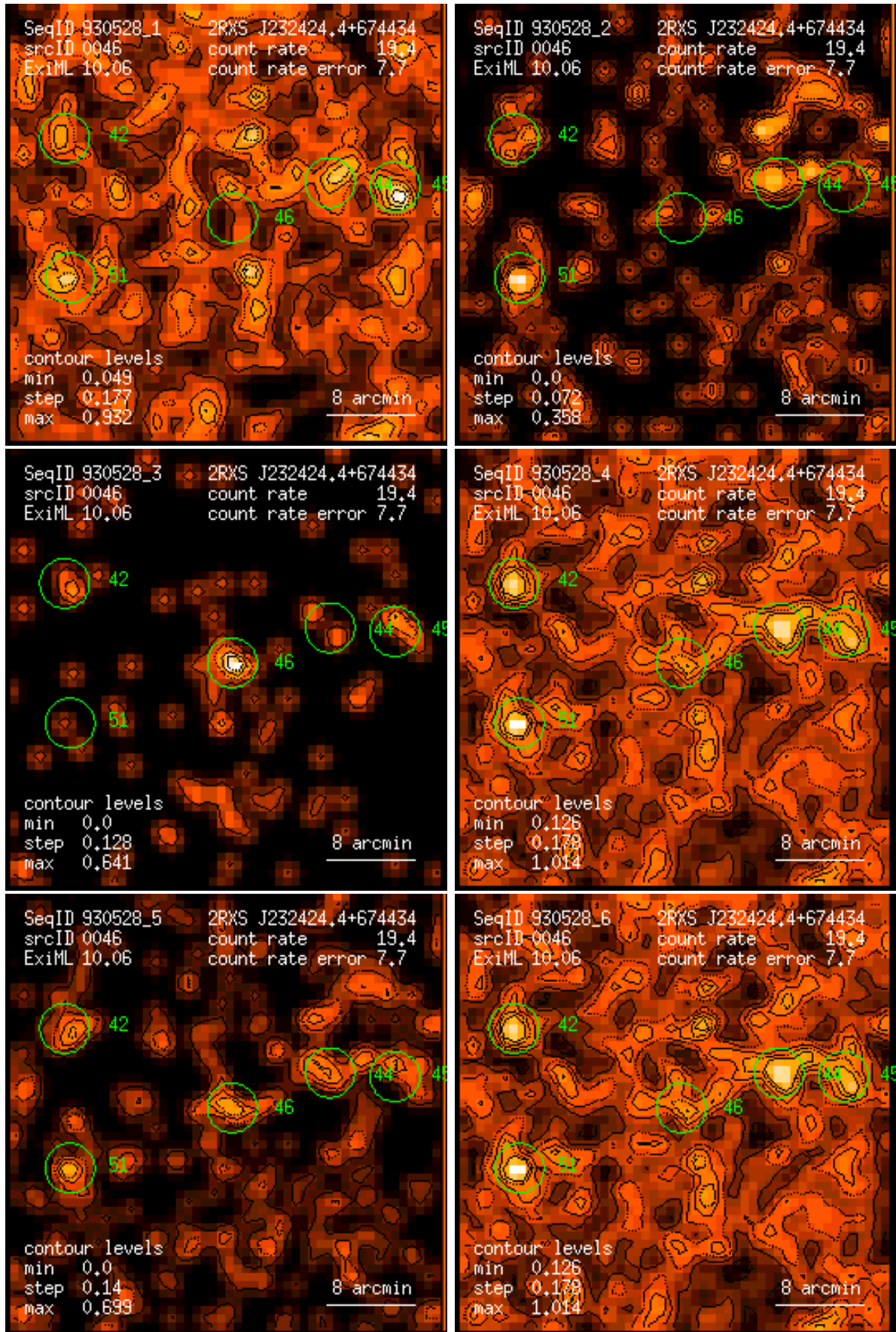
Figure 46: RASS 930528: detection 0046: band rate images, Gaussian filter: (1) PSPC channels 11 – 41, (2) 52 – 90, (3) 91 – 201, (4) 11 – 235, (5) 52 – 201, (6) 11 – 201. Broad band rates in counts/ks. Band rate contour levels in counts/ks/arcmin 2 .
