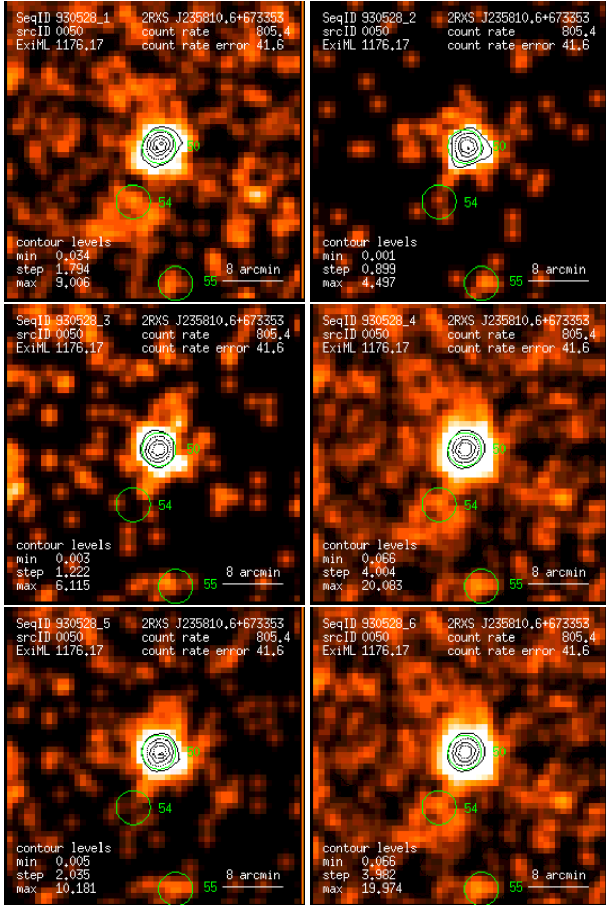
Figure 50: RASS 930528: detection 0050: band rate images, Gaussian filter: (1) PSPC channels 11 – 41, (2) 52 – 90, (3) 91 – 201, (4) 11 – 235, (5) 52 – 201, (6) 11 – 201. Broad band rates in counts/ks. Band rate contour levels in counts/ks/arcmin 2 .
