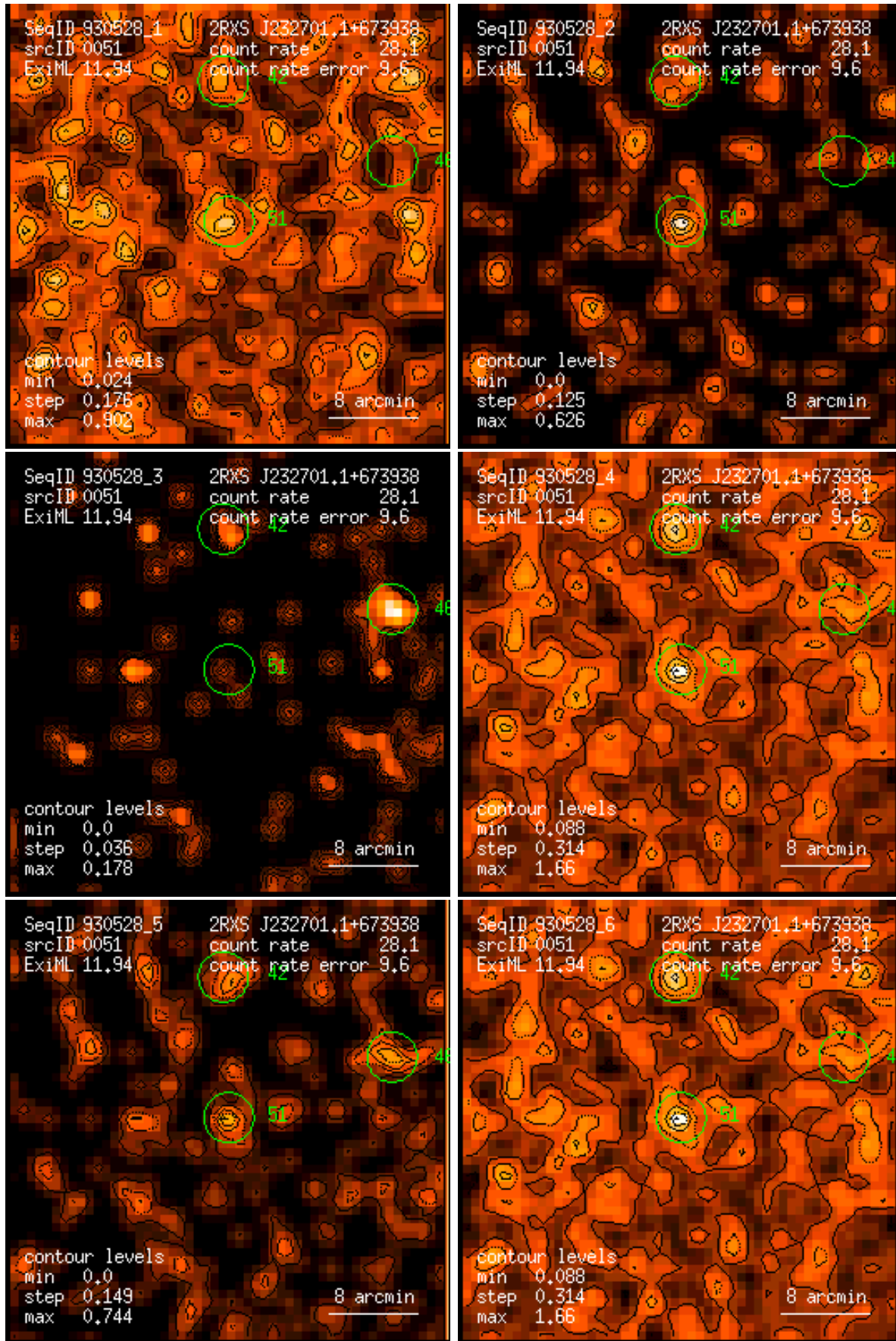
Figure 51: RASS 930528: detection 0051: band rate images, Gaussian filter: (1) PSPC channels 11 – 41, (2) 52 – 90, (3) 91 – 201, (4) 11 – 235, (5) 52 – 201, (6) 11 – 201. Broad band rates in counts/ks. Band rate contour levels in counts/ks/arcmin 2 .
