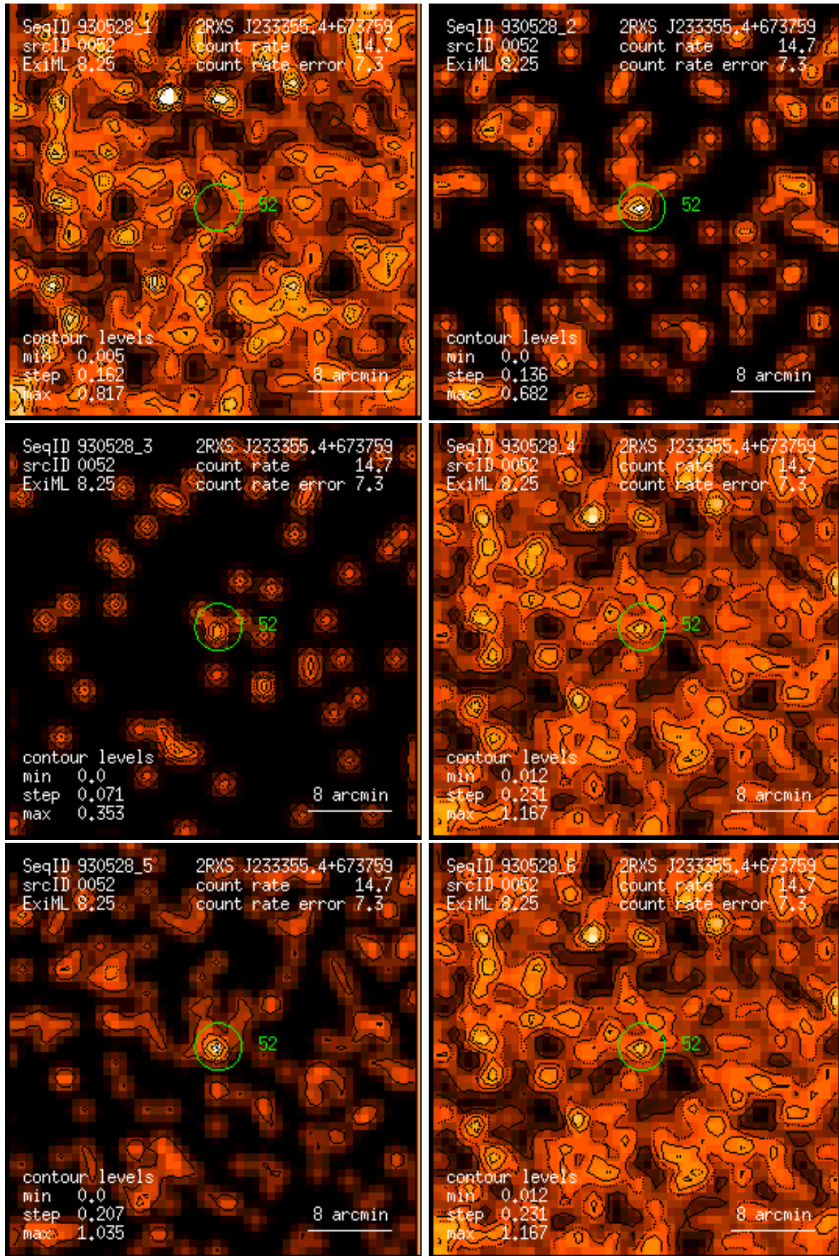
Figure 52: RASS 930528: detection 0052: band rate images, Gaussian filter: (1) PSPC channels 11 – 41, (2) 52 – 90, (3) 91 – 201, (4) 11 – 235, (5) 52 – 201, (6) 11 – 201. Broad band rates in counts/ks. Band rate contour levels in counts/ks/arcmin 2 .
