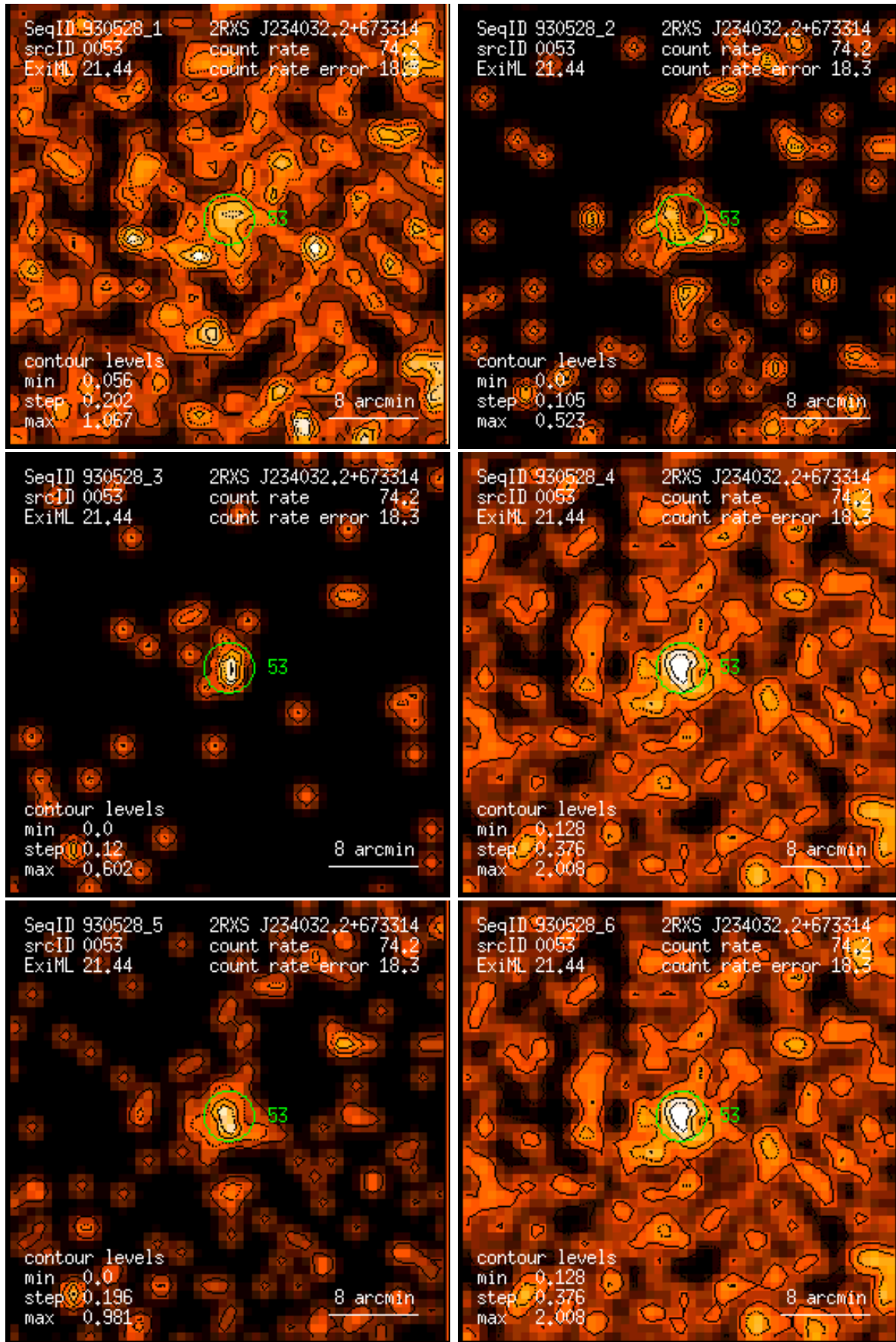
Figure 53: RASS 930528: detection 0053: band rate images, Gaussian filter: (1) PSPC channels 11 – 41, (2) 52 – 90, (3) 91 – 201, (4) 11 – 235, (5) 52 – 201, (6) 11 – 201. Broad band rates in counts/ks. Band rate contour levels in counts/ks/arcmin 2 .
