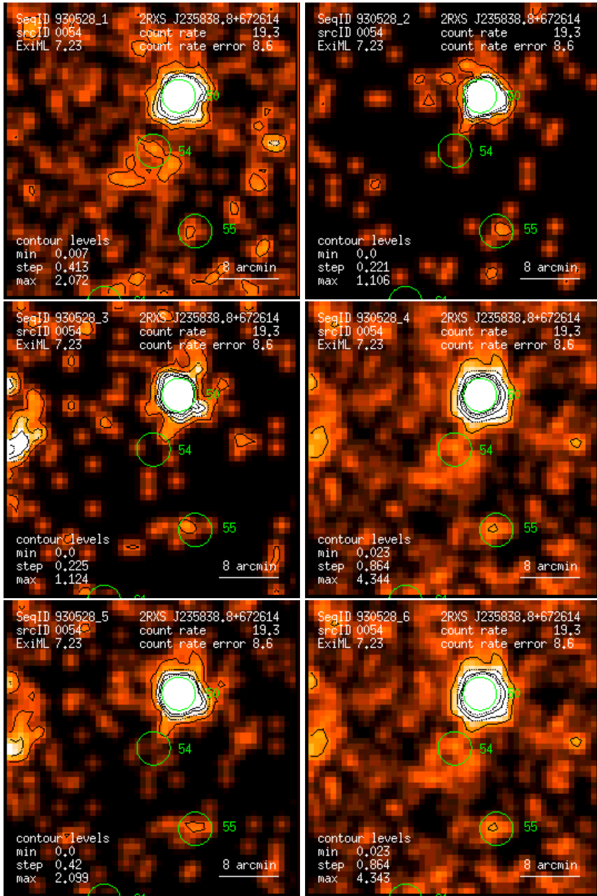
Figure 54: RASS 930528: detection 0054: band rate images, Gaussian filter: (1) PSPC channels 11 – 41, (2) 52 – 90, (3) 91 – 201, (4) 11 – 235, (5) 52 – 201, (6) 11 – 201. Broad band rates in counts/ks. Band rate contour levels in counts/ks/arcmin 2 .
