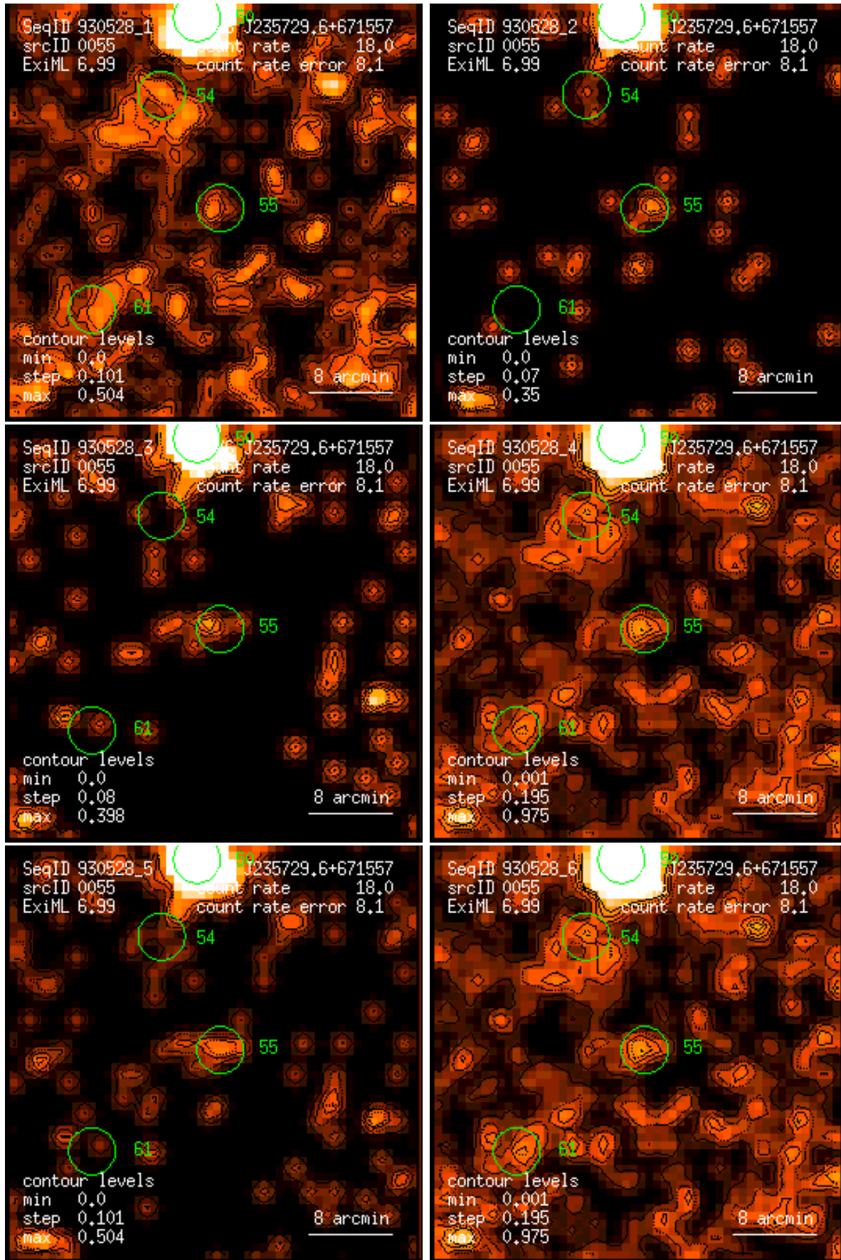
Figure 55: RASS 930528: detection 0055: band rate images, Gaussian filter: (1) PSPC channels 11 – 41, (2) 52 – 90, (3) 91 – 201, (4) 11 – 235, (5) 52 – 201, (6) 11 – 201. Broad band rates in counts/ks. Band rate contour levels in counts/ks/arcmin 2 .
