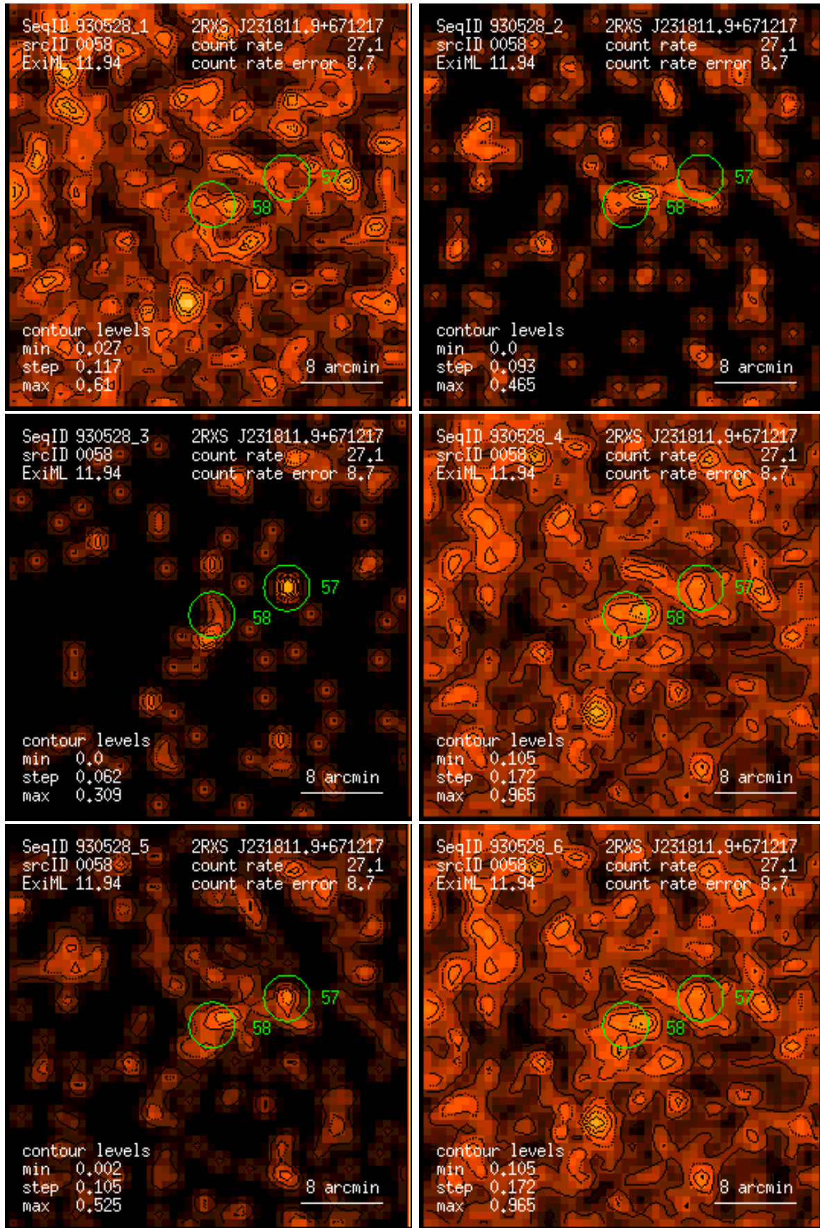
Figure 58: RASS 930528: detection 0058: band rate images, Gaussian filter: (1) PSPC channels 11 – 41, (2) 52 – 90, (3) 91 – 201, (4) 11 – 235, (5) 52 – 201, (6) 11 – 201. Broad band rates in counts/ks. Band rate contour levels in counts/ks/arcmin 2 .
