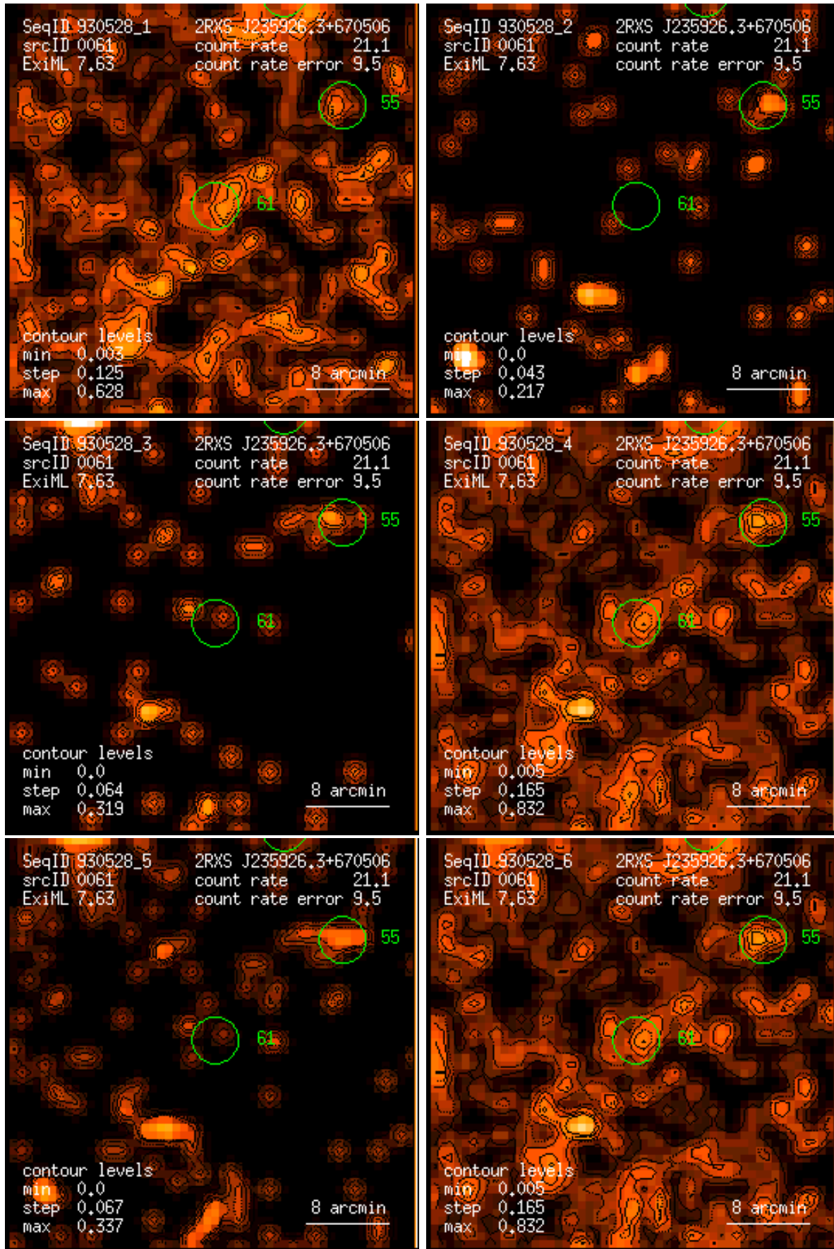
Figure 61: RASS 930528: detection 0061: band rate images, Gaussian filter: (1) PSPC channels 11 – 41, (2) 52 – 90, (3) 91 – 201, (4) 11 – 235, (5) 52 – 201, (6) 11 – 201. Broad band rates in counts/ks. Band rate contour levels in counts/ks/arcmin 2 .
