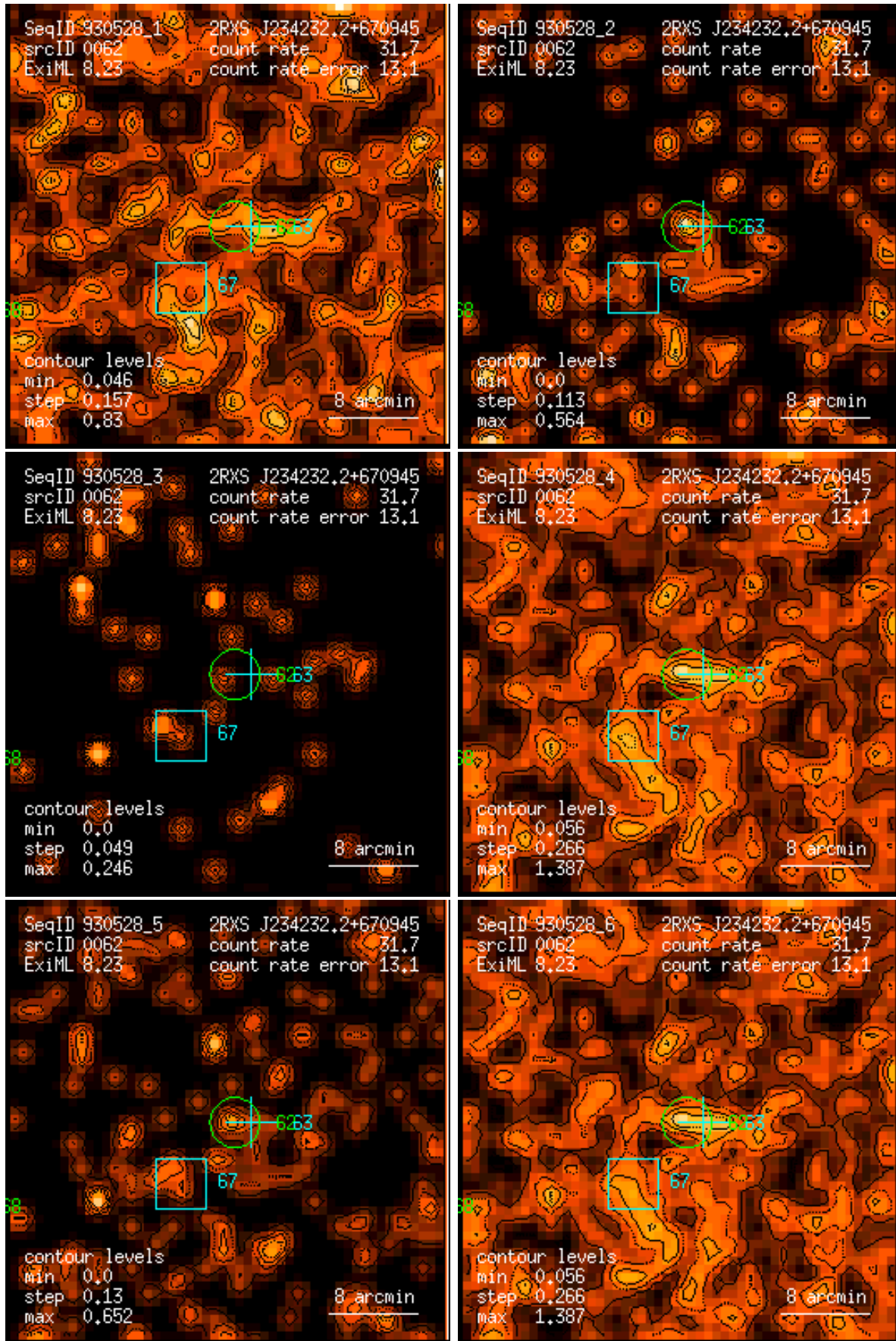
Figure 62: RASS 930528: detection 0062: band rate images, Gaussian filter: (1) PSPC channels 11 – 41, (2) 52 – 90, (3) 91 – 201, (4) 11 – 235, (5) 52 – 201, (6) 11 – 201. Broad band rates in counts/ks. Band rate contour levels in counts/ks/arcmin 2 .
