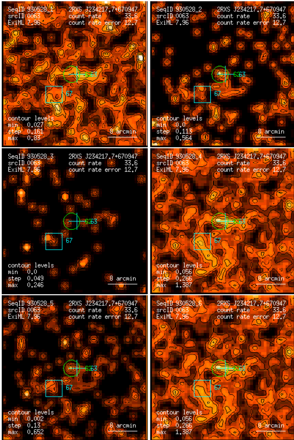
Figure 63: RASS 930528: detection 0063: band rate images, Gaussian filter: (1) PSPC channels 11 – 41, (2) 52 – 90, (3) 91 – 201, (4) 11 – 235, (5) 52 – 201, (6) 11 – 201. Broad band rates in counts/ks. Band rate contour levels in counts/ks/arcmin 2 .
