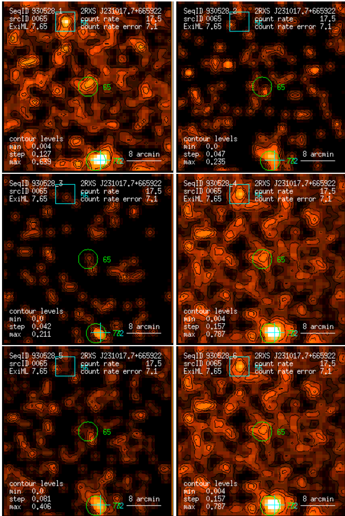
Figure 65: RASS 930528: detection 0065: band rate images, Gaussian filter: (1) PSPC channels 11 – 41, (2) 52 – 90, (3) 91 – 201, (4) 11 – 235, (5) 52 – 201, (6) 11 – 201. Broad band rates in counts/ks. Band rate contour levels in counts/ks/arcmin 2 .
