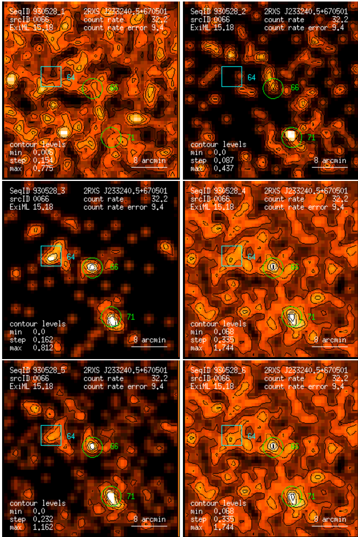
Figure 66: RASS 930528: detection 0066: band rate images, Gaussian filter: (1) PSPC channels 11 – 41, (2) 52 – 90, (3) 91 – 201, (4) 11 – 235, (5) 52 – 201, (6) 11 – 201. Broad band rates in counts/ks. Band rate contour levels in counts/ks/arcmin 2 .
