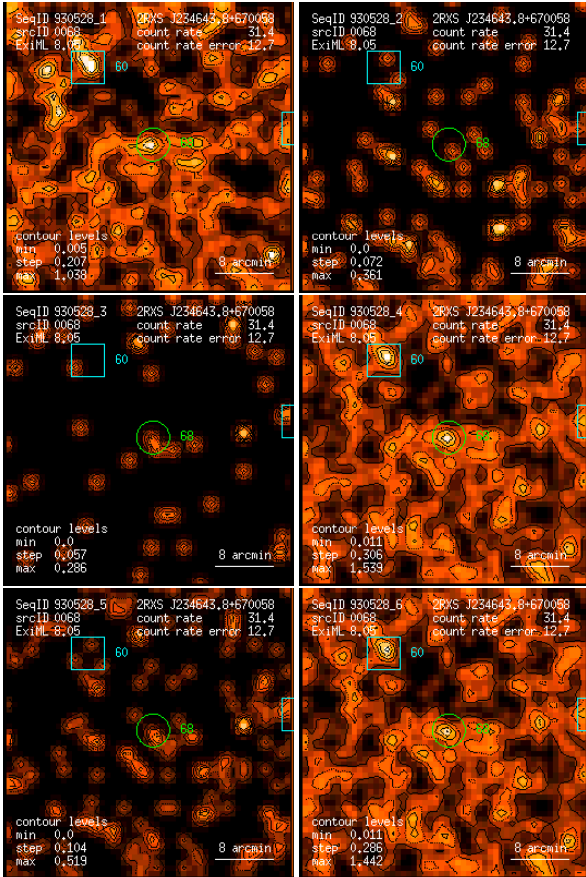
Figure 68: RASS 930528: detection 0068: band rate images, Gaussian filter: (1) PSPC channels 11 – 41, (2) 52 – 90, (3) 91 – 201, (4) 11 – 235, (5) 52 – 201, (6) 11 – 201. Broad band rates in counts/ks. Band rate contour levels in counts/ks/arcmin 2 .
