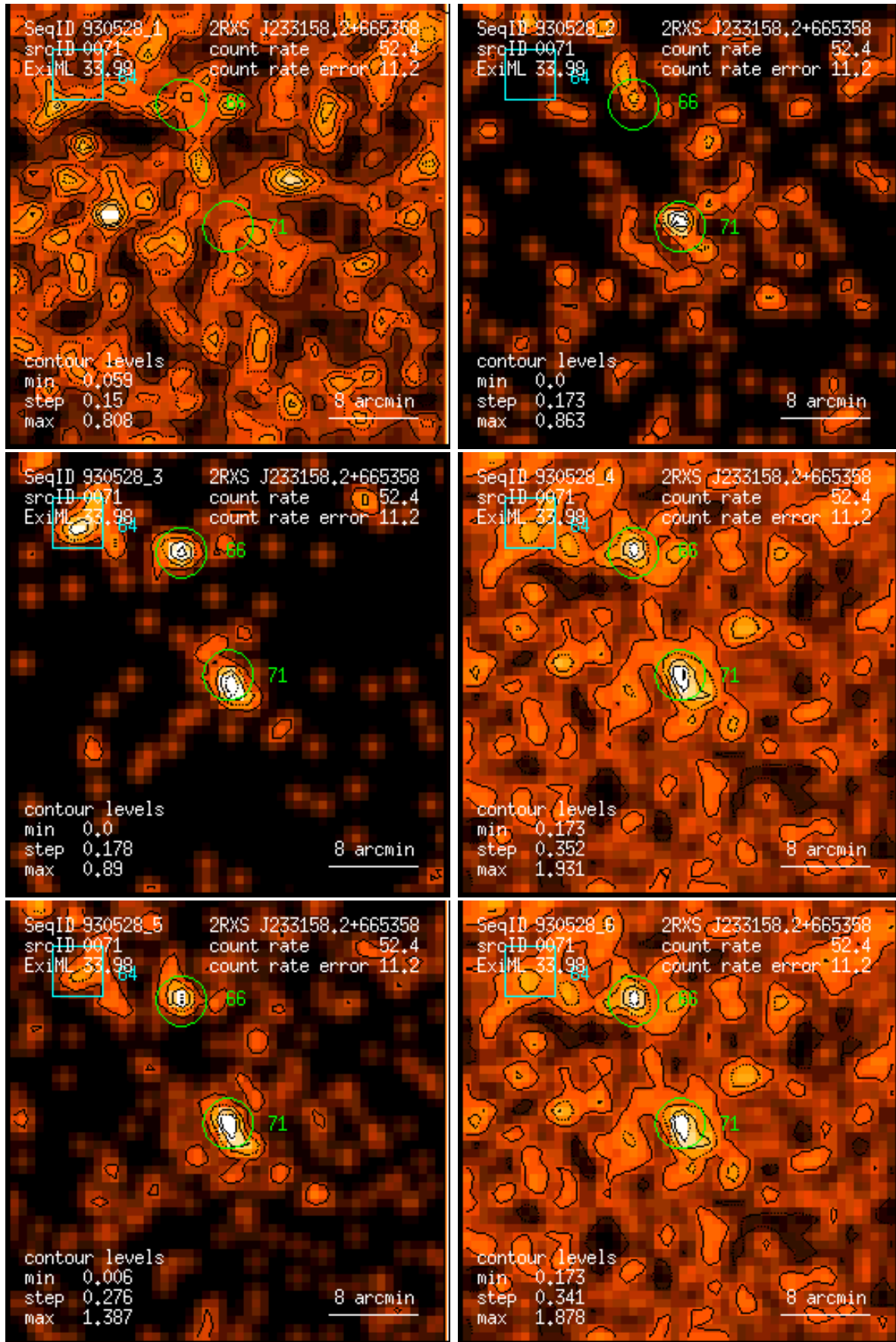
Figure 71: RASS 930528: detection 0071: band rate images, Gaussian filter: (1) PSPC channels 11 – 41, (2) 52 – 90, (3) 91 – 201, (4) 11 – 235, (5) 52 – 201, (6) 11 – 201. Broad band rates in counts/ks. Band rate contour levels in counts/ks/arcmin 2 .
