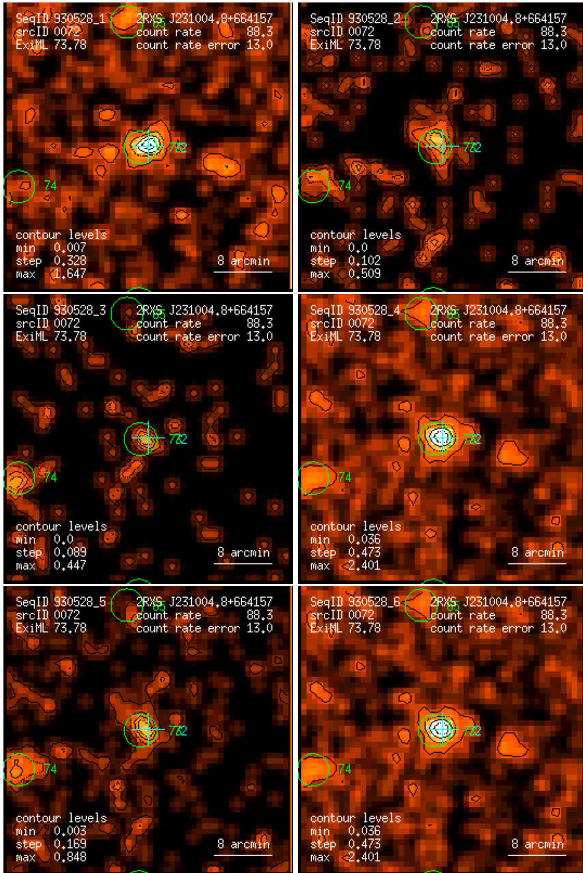
Figure 72: RASS 930528: detection 0072: band rate images, Gaussian filter: (1) PSPC channels 11 – 41, (2) 52 – 90, (3) 91 – 201, (4) 11 – 235, (5) 52 – 201, (6) 11 – 201. Broad band rates in counts/ks. Band rate contour levels in counts/ks/arcmin 2 .
