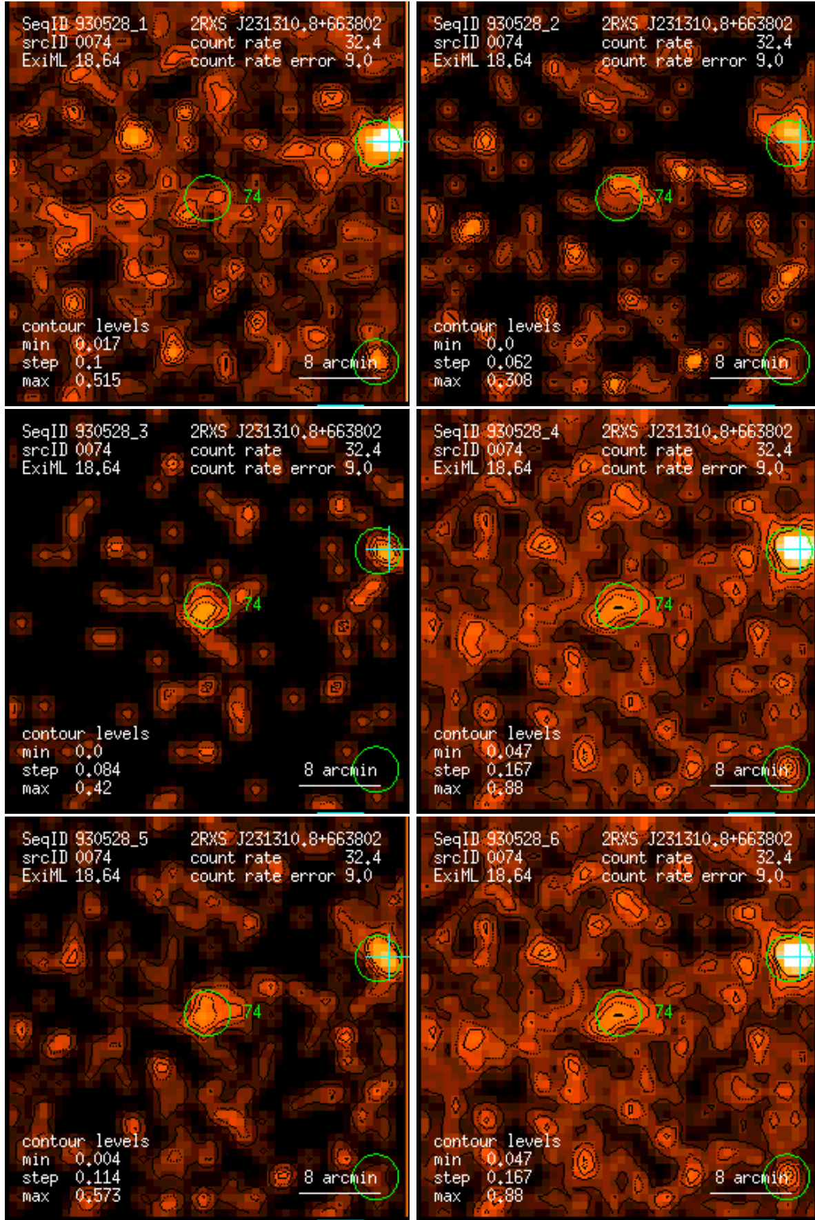
Figure 74: RASS 930528: detection 0074: band rate images, Gaussian filter: (1) PSPC channels 11 – 41, (2) 52 – 90, (3) 91 – 201, (4) 11 – 235, (5) 52 – 201, (6) 11 – 201. Broad band rates in counts/ks. Band rate contour levels in counts/ks/arcmin 2 .
