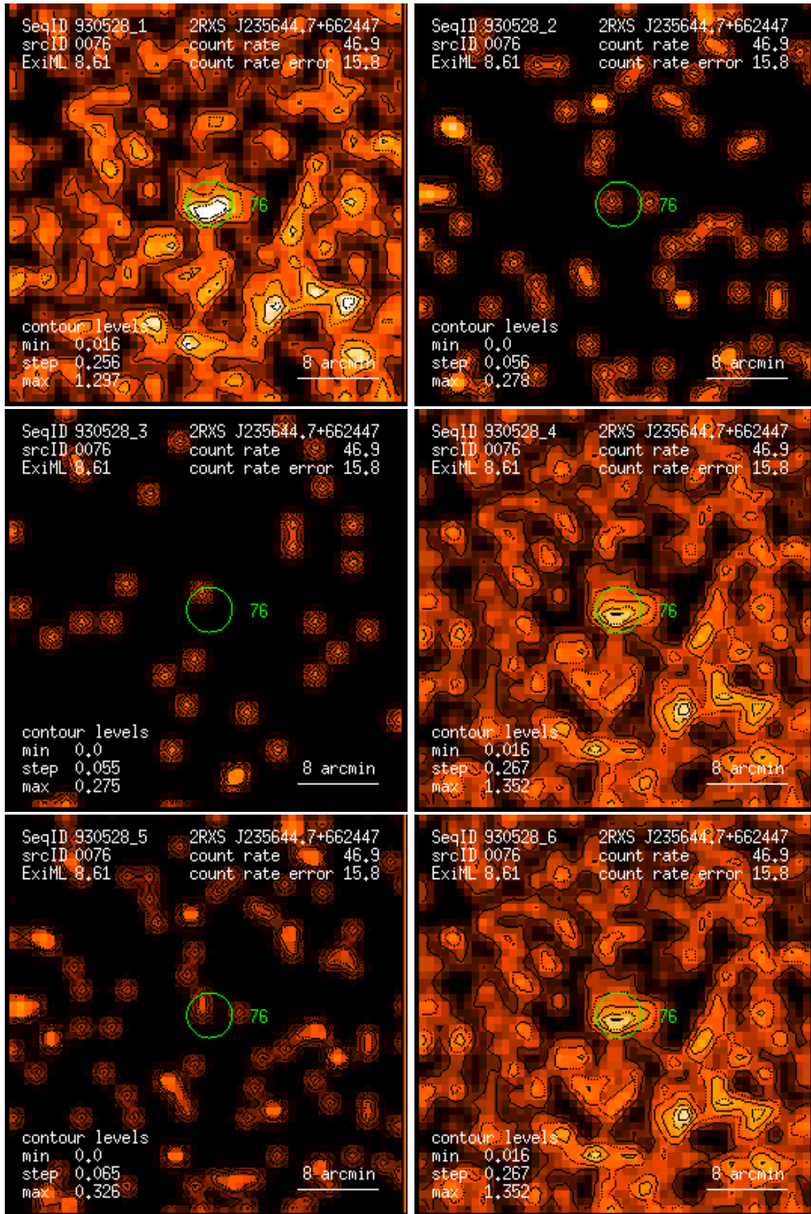
Figure 76: RASS 930528: detection 0076: band rate images, Gaussian filter: (1) PSPC channels 11 – 41, (2) 52 – 90, (3) 91 – 201, (4) 11 – 235, (5) 52 – 201, (6) 11 – 201. Broad band rates in counts/ks. Band rate contour levels in counts/ks/arcmin 2 .
