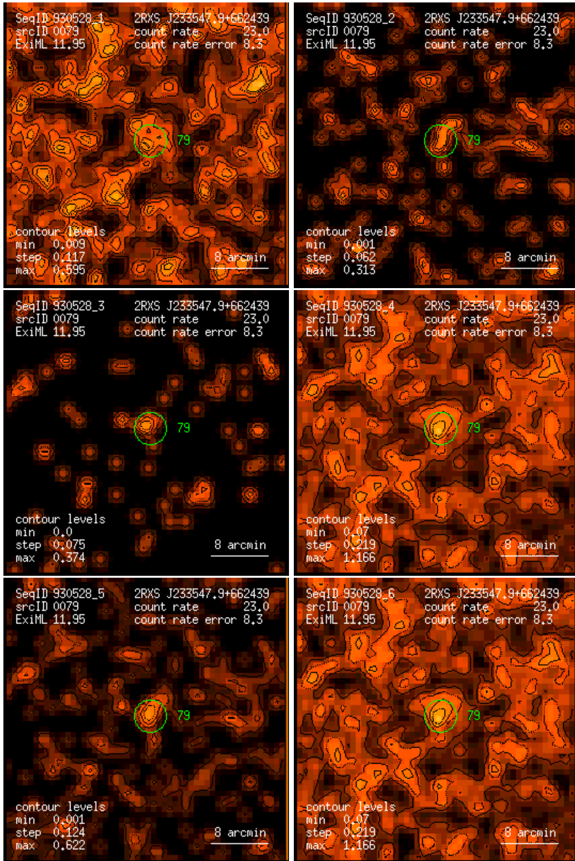
Figure 79: RASS 930528: detection 0079: band rate images, Gaussian filter: (1) PSPC channels 11 – 41, (2) 52 – 90, (3) 91 – 201, (4) 11 – 235, (5) 52 – 201, (6) 11 – 201. Broad band rates in counts/ks. Band rate contour levels in counts/ks/arcmin 2 .
