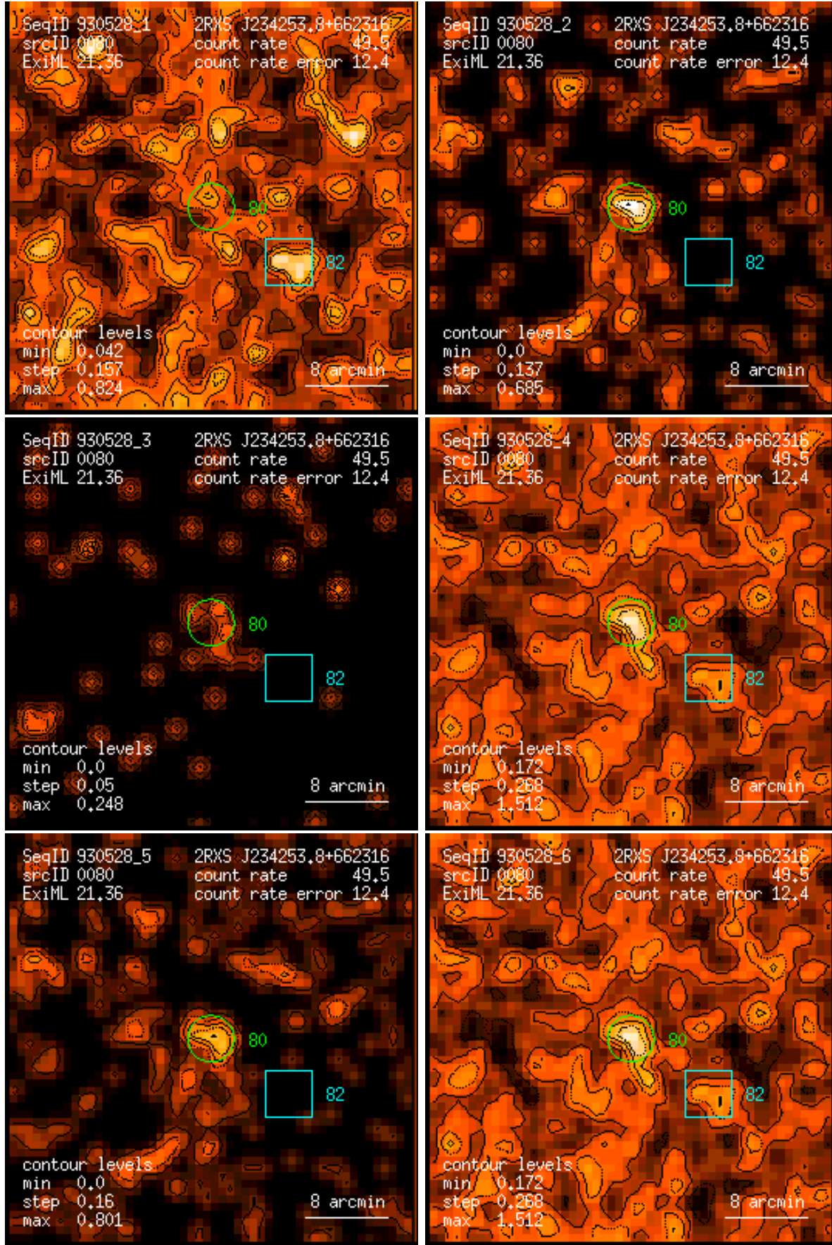
Figure 80: RASS 930528: detection 0080: band rate images, Gaussian filter: (1) PSPC channels 11 – 41, (2) 52 – 90, (3) 91 – 201, (4) 11 – 235, (5) 52 – 201, (6) 11 – 201. Broad band rates in counts/ks. Band rate contour levels in counts/ks/arcmin 2 .
