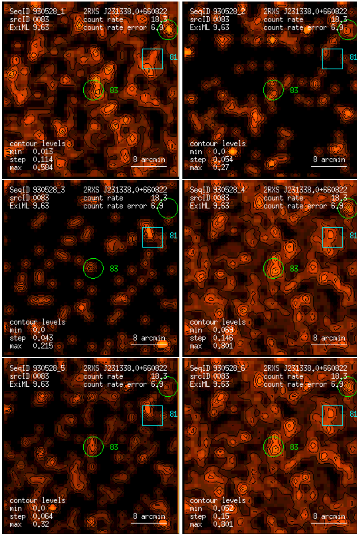
Figure 83: RASS 930528: detection 0083: band rate images, Gaussian filter: (1) PSPC channels 11 – 41, (2) 52 – 90, (3) 91 – 201, (4) 11 – 235, (5) 52 – 201, (6) 11 – 201. Broad band rates in counts/ks. Band rate contour levels in counts/ks/arcmin 2 .
