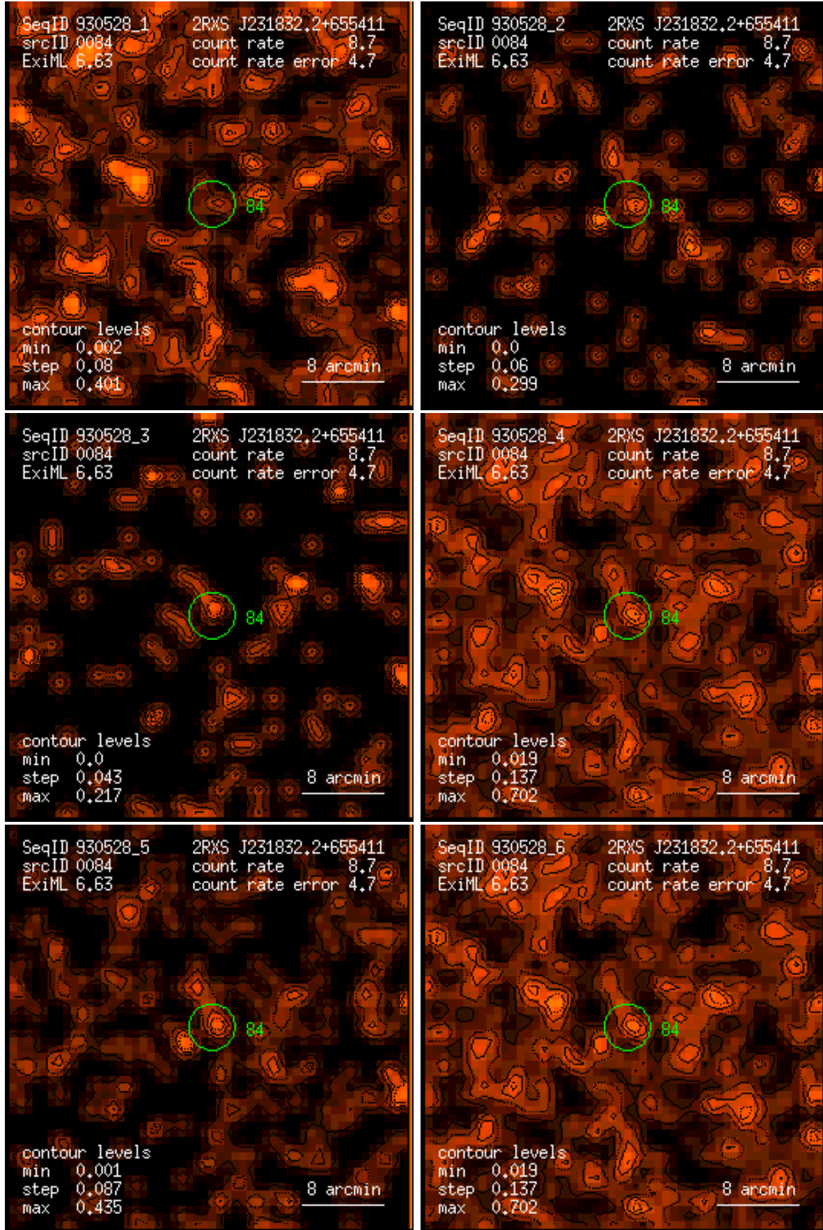
Figure 84: RASS 930528: detection 0084: band rate images, Gaussian filter: (1) PSPC channels 11 – 41, (2) 52 – 90, (3) 91 – 201, (4) 11 – 235, (5) 52 – 201, (6) 11 – 201. Broad band rates in counts/ks. Band rate contour levels in counts/ks/arcmin 2 .
