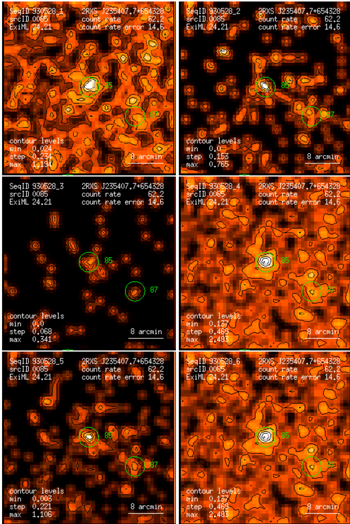
Figure 85: RASS 930528: detection 0085: band rate images, Gaussian filter: (1) PSPC channels 11 – 41, (2) 52 – 90, (3) 91 – 201, (4) 11 – 235, (5) 52 – 201, (6) 11 – 201. Broad band rates in counts/ks. Band rate contour levels in counts/ks/arcmin 2 .
