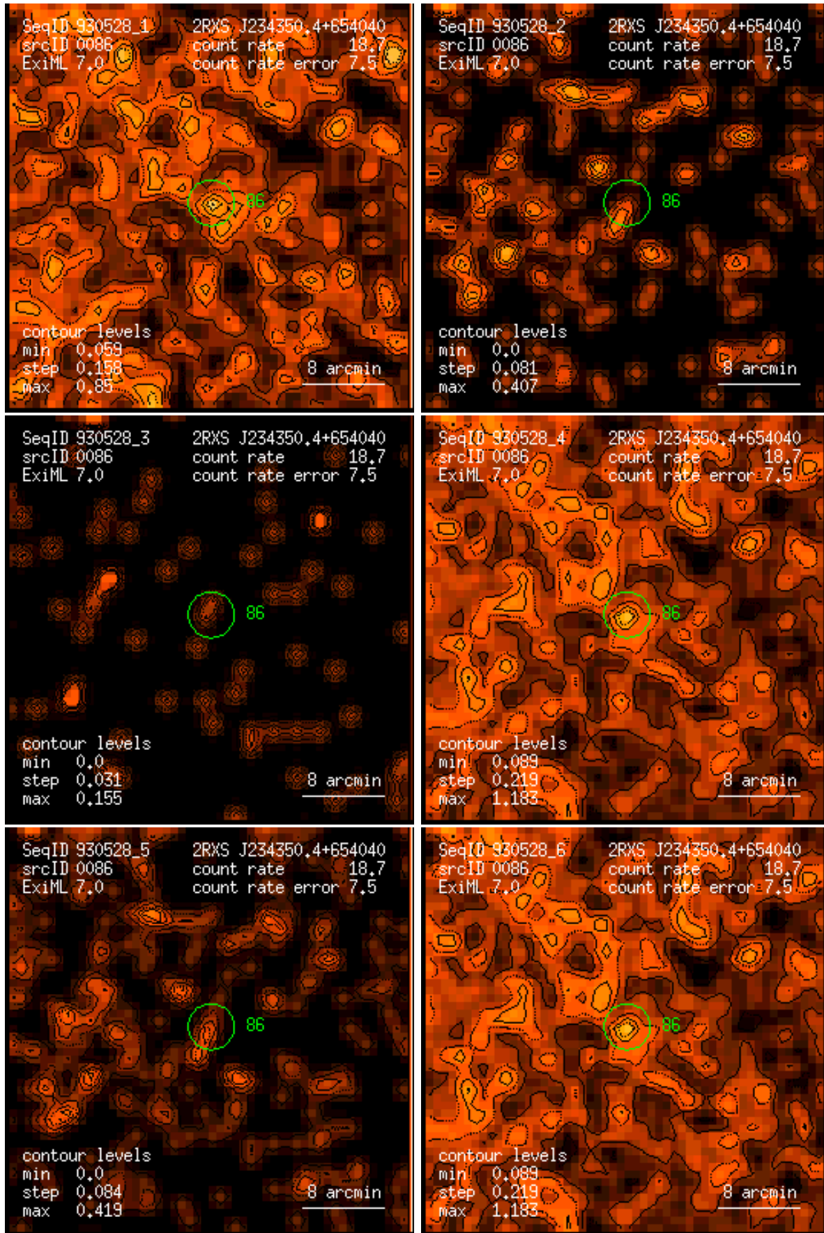
Figure 86: RASS 930528: detection 0086: band rate images, Gaussian filter: (1) PSPC channels 11 – 41, (2) 52 – 90, (3) 91 – 201, (4) 11 – 235, (5) 52 – 201, (6) 11 – 201. Broad band rates in counts/ks. Band rate contour levels in counts/ks/arcmin 2 .
