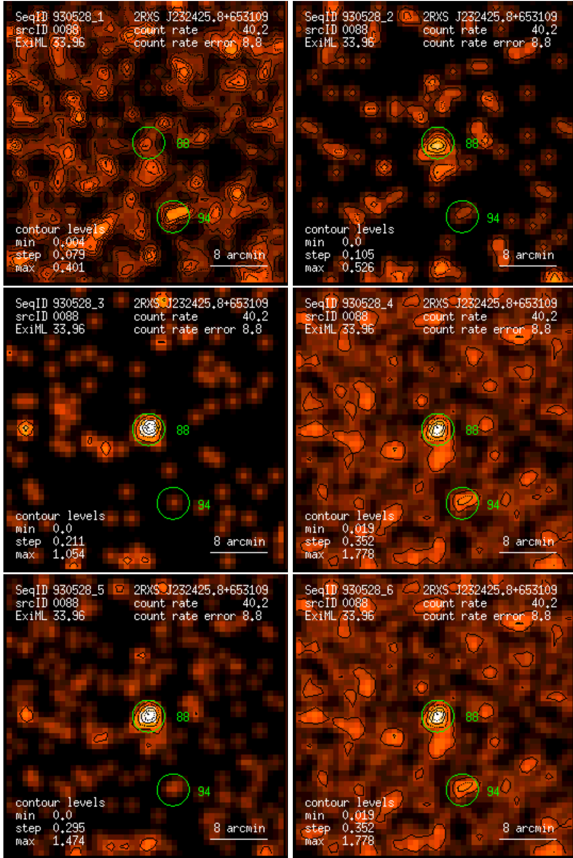
Figure 88: RASS 930528: detection 0088: band rate images, Gaussian filter: (1) PSPC channels 11 – 41, (2) 52 – 90, (3) 91 – 201, (4) 11 – 235, (5) 52 – 201, (6) 11 – 201. Broad band rates in counts/ks. Band rate contour levels in counts/ks/arcmin 2 .
