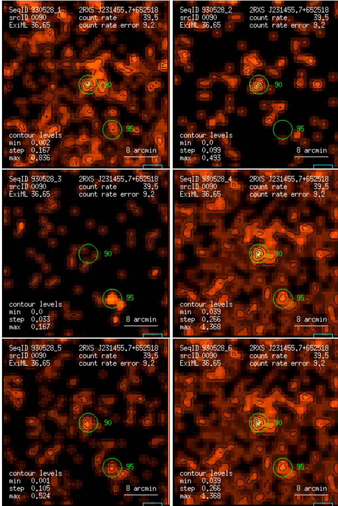
Figure 90: RASS 930528: detection 0090: band rate images, Gaussian filter: (1) PSPC channels 11 – 41, (2) 52 – 90, (3) 91 – 201, (4) 11 – 235, (5) 52 – 201, (6) 11 – 201. Broad band rates in counts/ks. Band rate contour levels in counts/ks/arcmin 2 .
