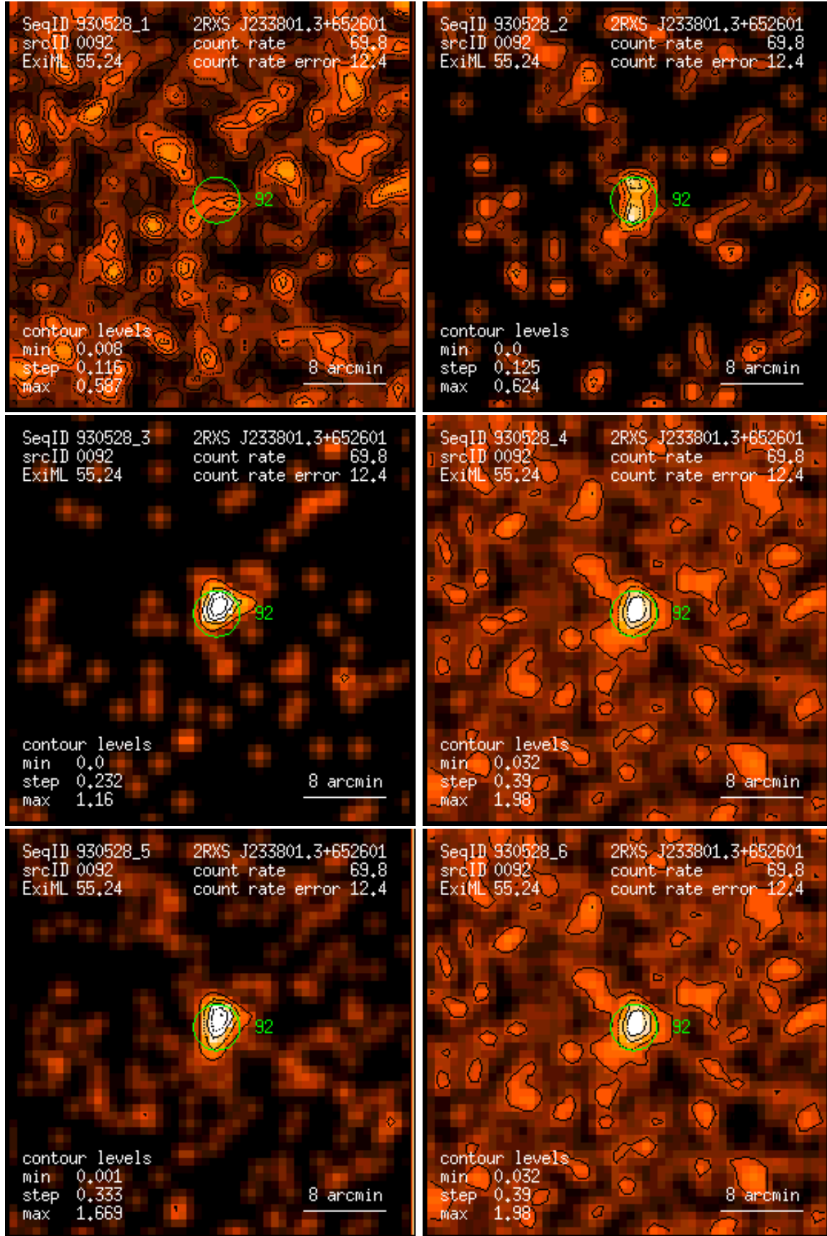
Figure 92: RASS 930528: detection 0092: band rate images, Gaussian filter: (1) PSPC channels 11 – 41, (2) 52 – 90, (3) 91 – 201, (4) 11 – 235, (5) 52 – 201, (6) 11 – 201. Broad band rates in counts/ks. Band rate contour levels in counts/ks/arcmin 2 .
