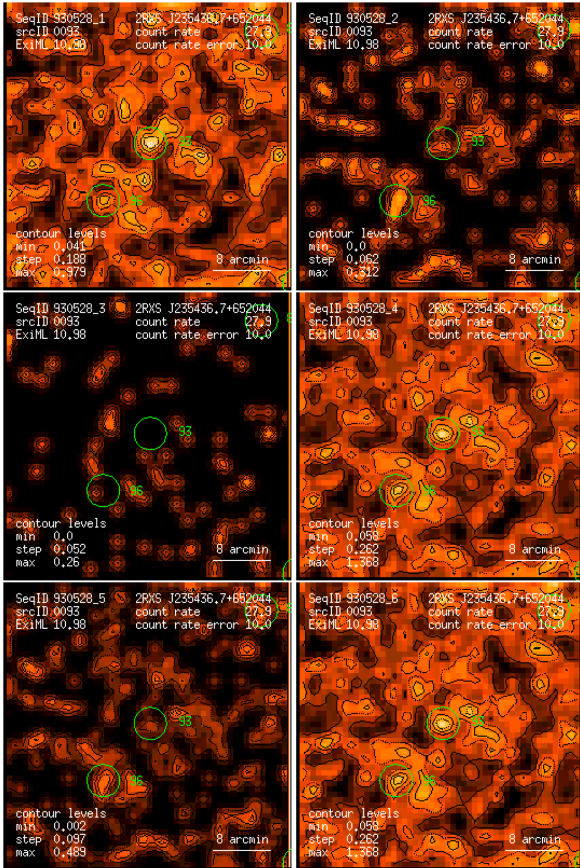
Figure 93: RASS 930528: detection 0093: band rate images, Gaussian filter: (1) PSPC channels 11 – 41, (2) 52 – 90, (3) 91 – 201, (4) 11 – 235, (5) 52 – 201, (6) 11 – 201. Broad band rates in counts/ks. Band rate contour levels in counts/ks/arcmin 2 .
