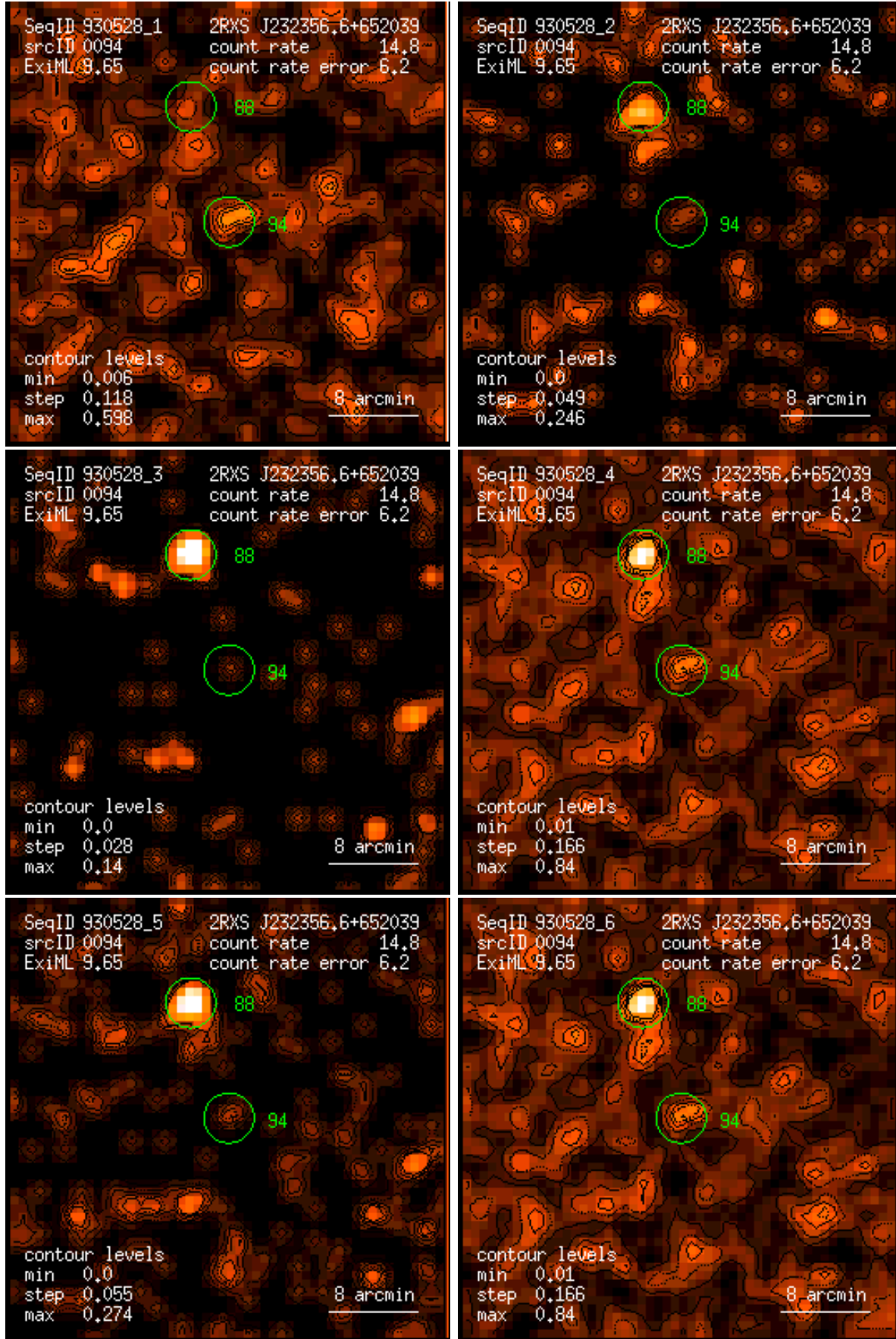
Figure 94: RASS 930528: detection 0094: band rate images, Gaussian filter: (1) PSPC channels 11 – 41, (2) 52 – 90, (3) 91 – 201, (4) 11 – 235, (5) 52 – 201, (6) 11 – 201. Broad band rates in counts/ks. Band rate contour levels in counts/ks/arcmin 2 .
