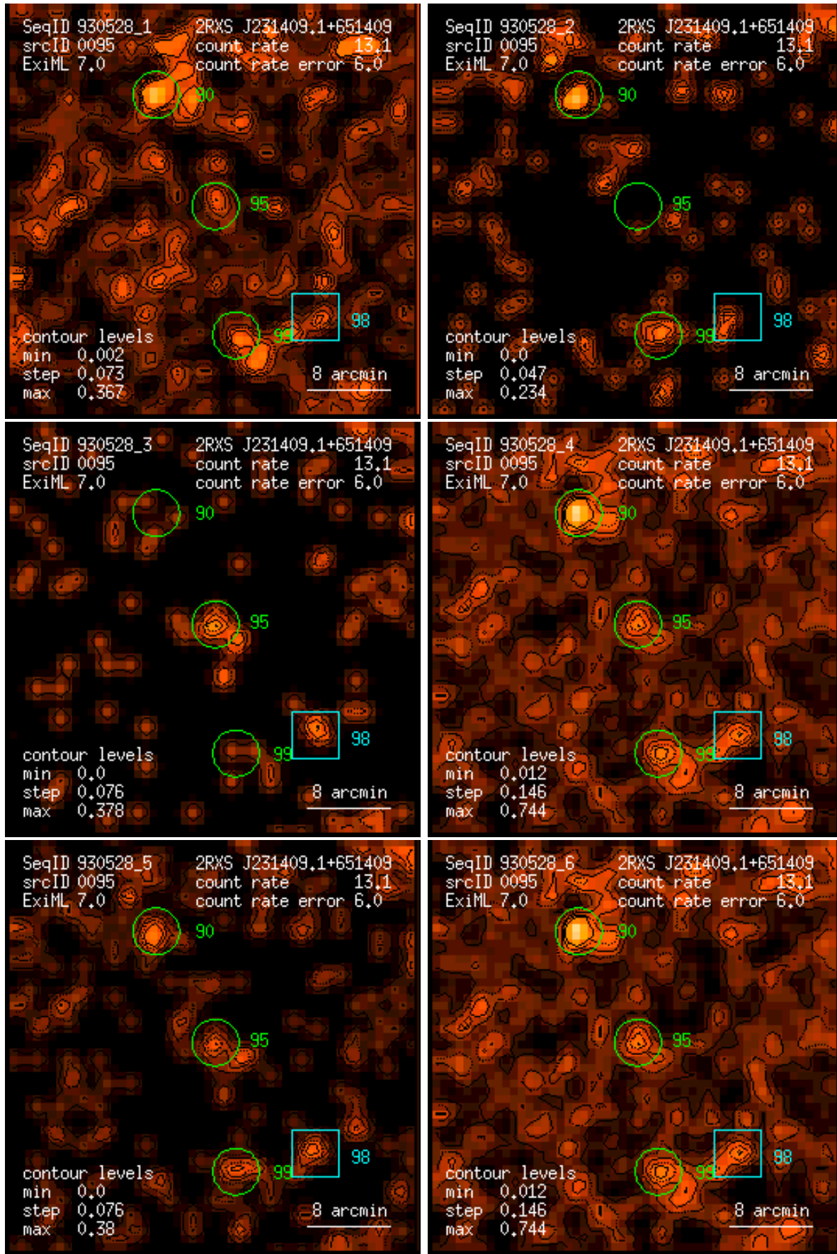
Figure 95: RASS 930528: detection 0095: band rate images, Gaussian filter: (1) PSPC channels 11 – 41, (2) 52 – 90, (3) 91 – 201, (4) 11 – 235, (5) 52 – 201, (6) 11 – 201. Broad band rates in counts/ks. Band rate contour levels in counts/ks/arcmin 2 .
