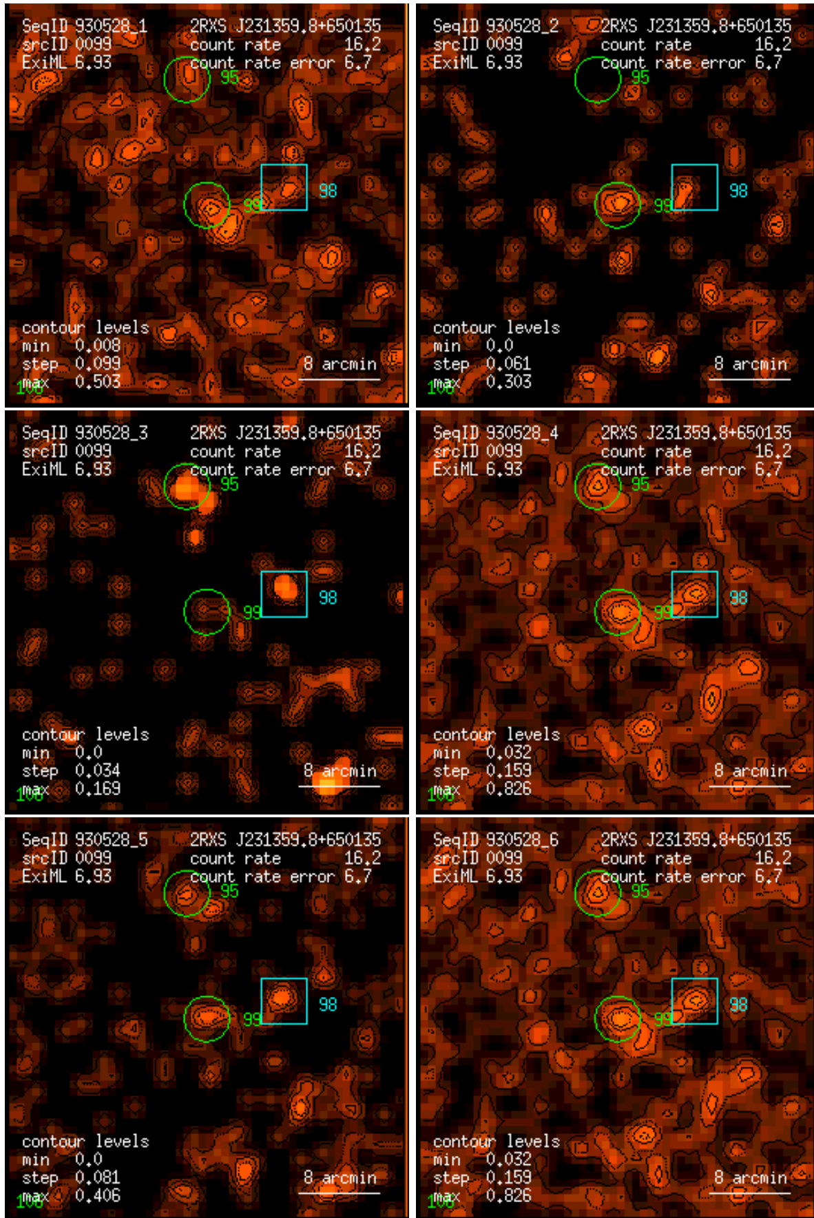
Figure 99: RASS 930528: detection 0099: band rate images, Gaussian filter: (1) PSPC channels 11 – 41, (2) 52 – 90, (3) 91 – 201, (4) 11 – 235, (5) 52 – 201, (6) 11 – 201. Broad band rates in counts/ks. Band rate contour levels in counts/ks/arcmin 2 .
