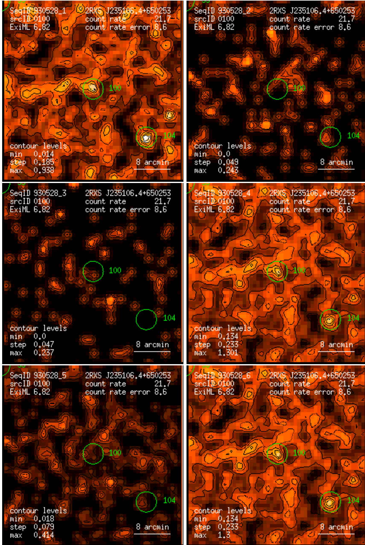
Figure 100: RASS 930528: detection 0100: band rate images, Gaussian filter: (1) PSPC channels 11 – 41, (2) 52 – 90, (3) 91 – 201, (4) 11 – 235, (5) 52 – 201, (6) 11 – 201. Broad band rates in counts/ks. Band rate contour levels in counts/ks/arcmin 2 .
