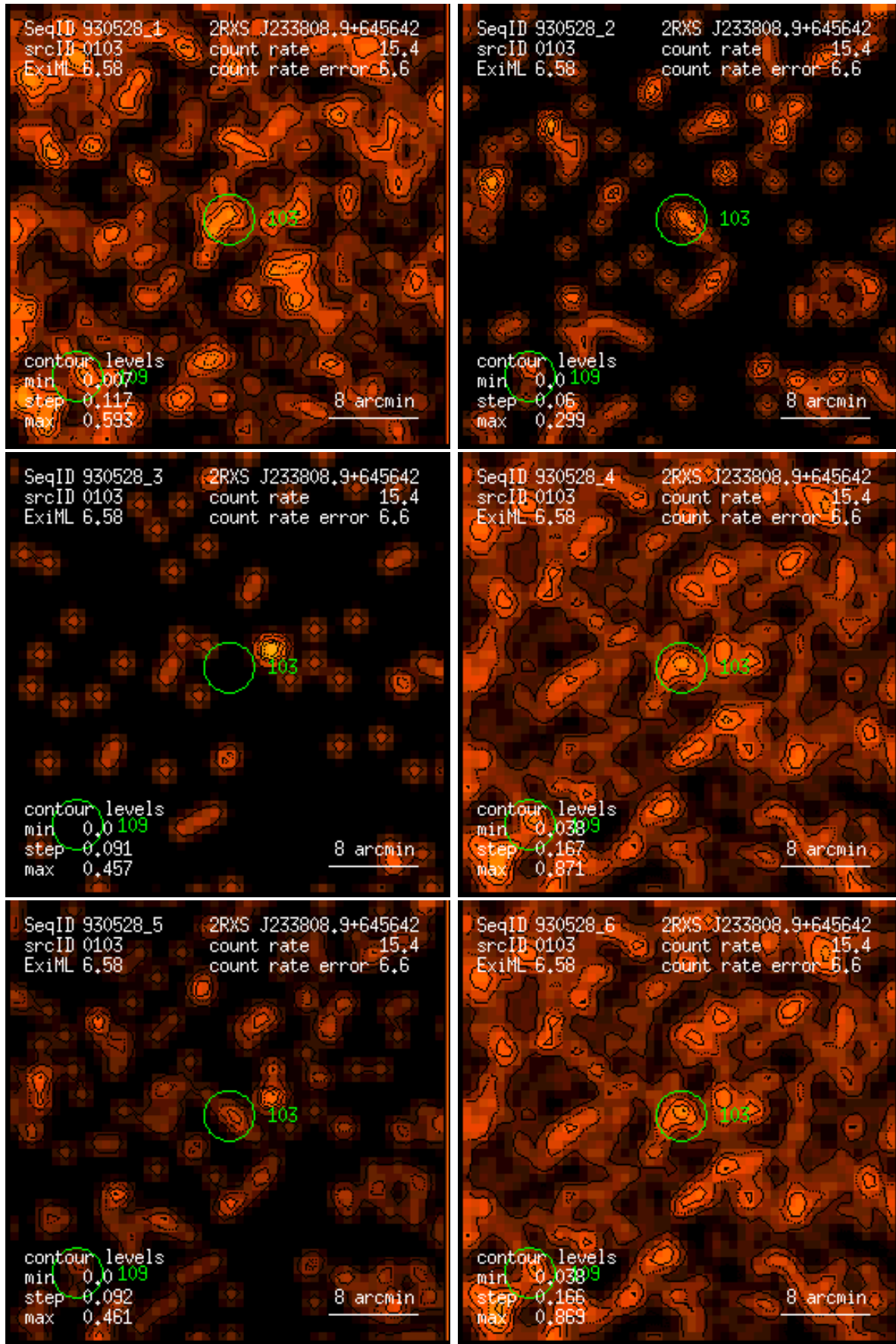
Figure 103: RASS 930528: detection 0103: band rate images, Gaussian filter: (1) PSPC channels 11 – 41, (2) 52 – 90, (3) 91 – 201, (4) 11 – 235, (5) 52 – 201, (6) 11 – 201. Broad band rates in counts/ks. Band rate contour levels in counts/ks/arcmin 2 .
