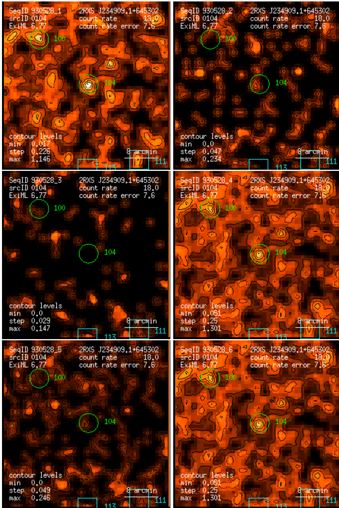
Figure 104: RASS 930528: detection 0104: band rate images, Gaussian filter: (1) PSPC channels 11 – 41, (2) 52 – 90, (3) 91 – 201, (4) 11 – 235, (5) 52 – 201, (6) 11 – 201. Broad band rates in counts/ks. Band rate contour levels in counts/ks/arcmin 2 .
