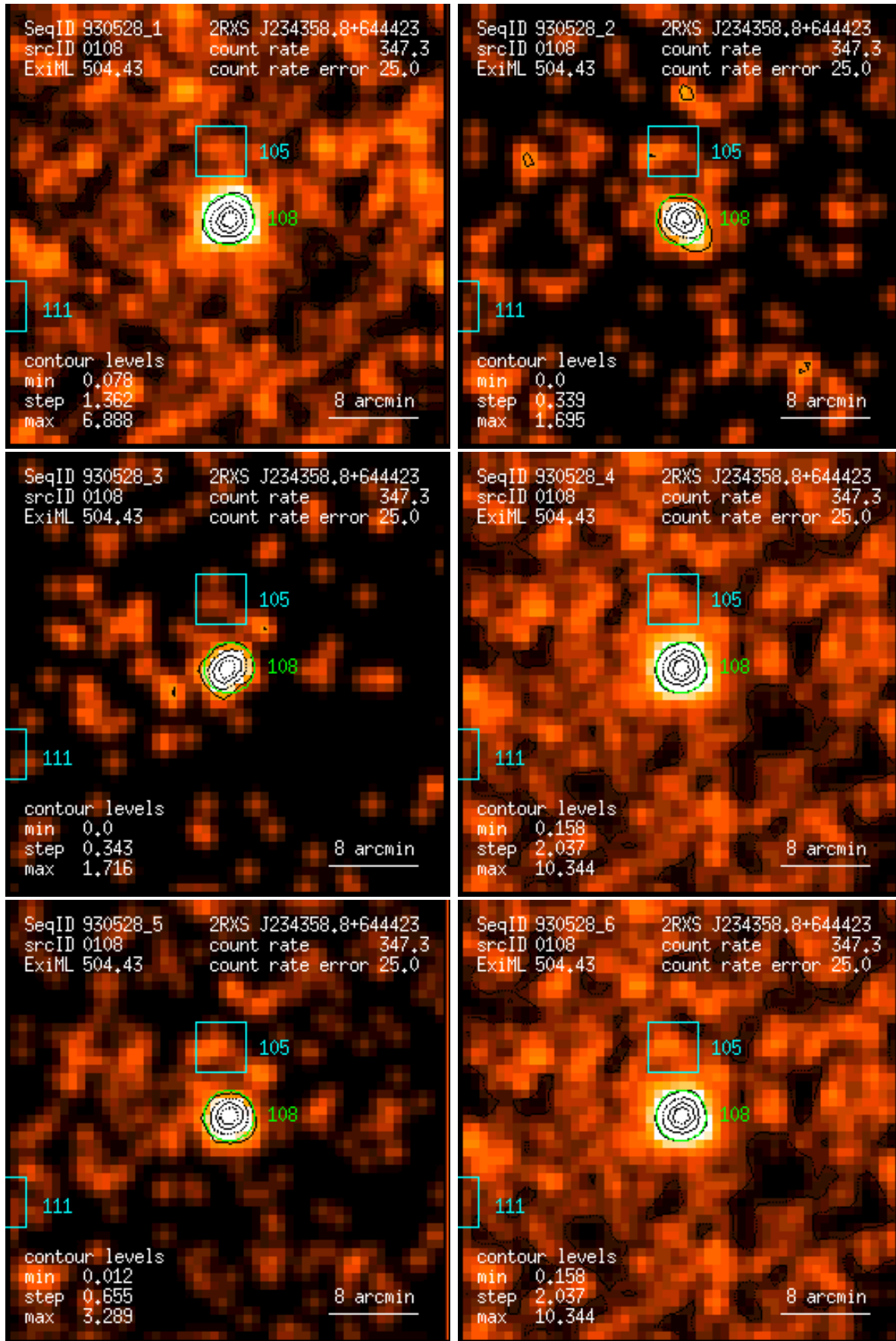
Figure 108: RASS 930528: detection 0108: band rate images, Gaussian filter: (1) PSPC channels 11 – 41, (2) 52 – 90, (3) 91 – 201, (4) 11 – 235, (5) 52 – 201, (6) 11 – 201. Broad band rates in counts/ks. Band rate contour levels in counts/ks/arcmin 2 .
