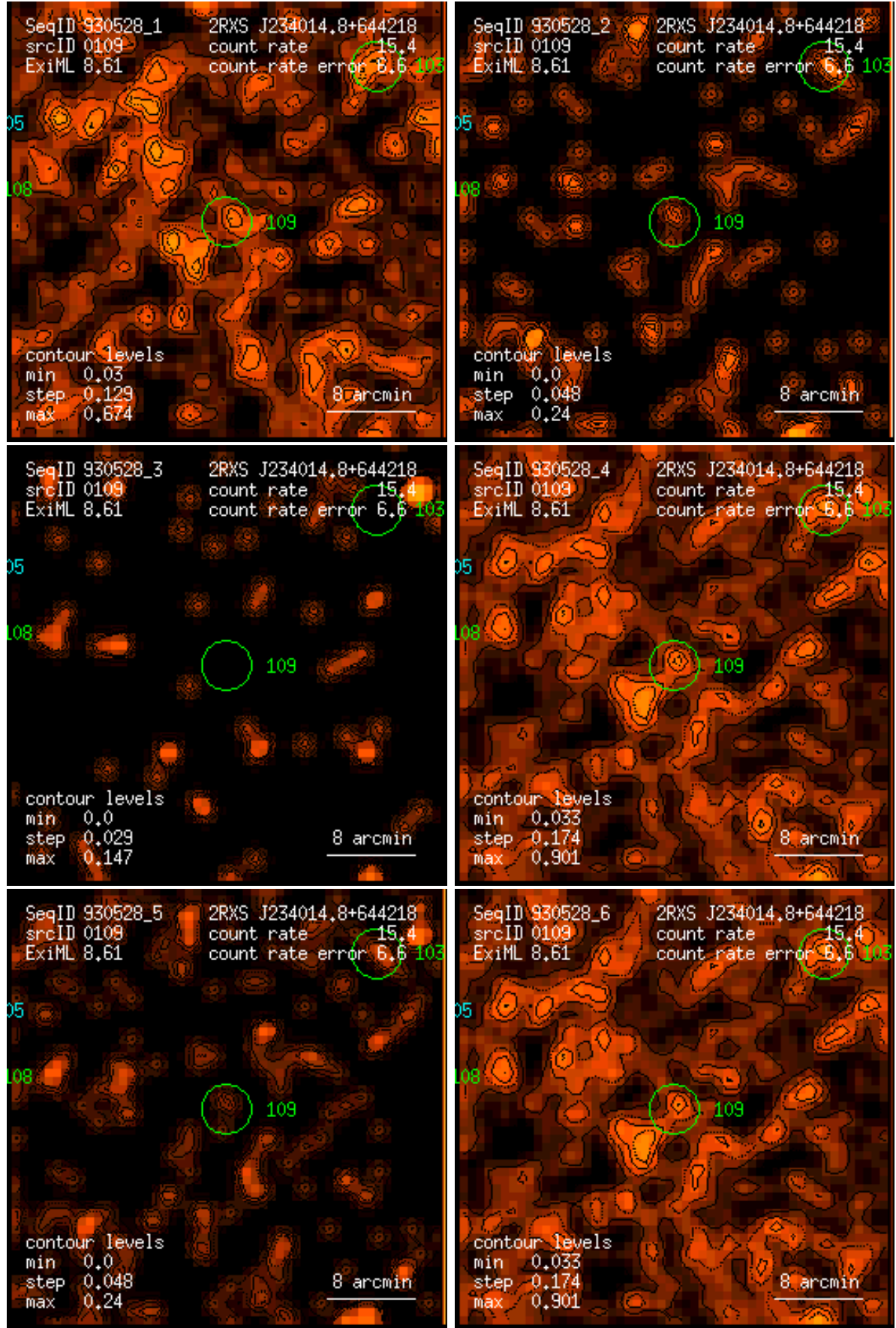
Figure 109: RASS 930528: detection 0109: band rate images, Gaussian filter: (1) PSPC channels 11 – 41, (2) 52 – 90, (3) 91 – 201, (4) 11 – 235, (5) 52 – 201, (6) 11 – 201. Broad band rates in counts/ks. Band rate contour levels in counts/ks/arcmin 2 .
