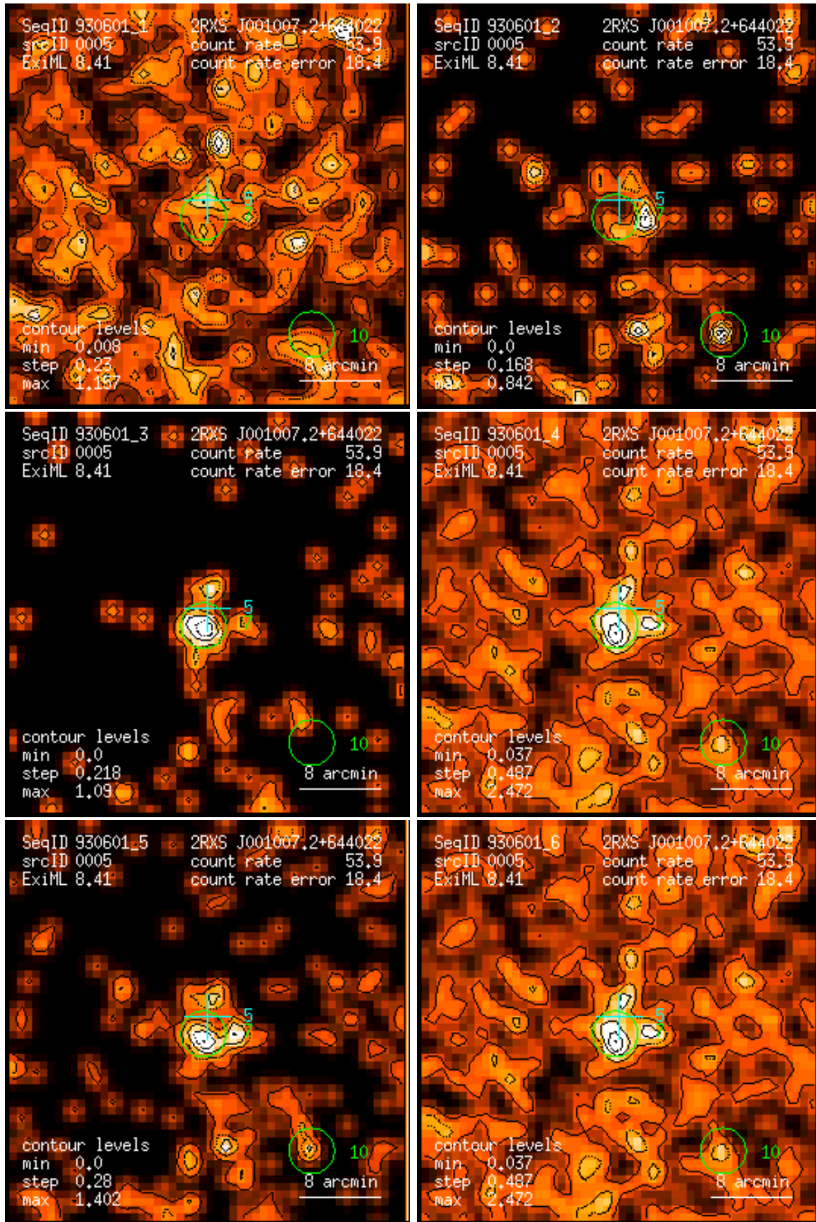
Figure 5: RASS 930601: detection 0005: band rate images, Gaussian filter: (1) PSPC channels 11 – 41, (2) 52 – 90, (3) 91 – 201, (4) 11 – 235, (5) 52 – 201, (6) 11 – 201. Broad band rates in counts/ks. Band rate contour levels in counts/ks/arcmin 2 .
