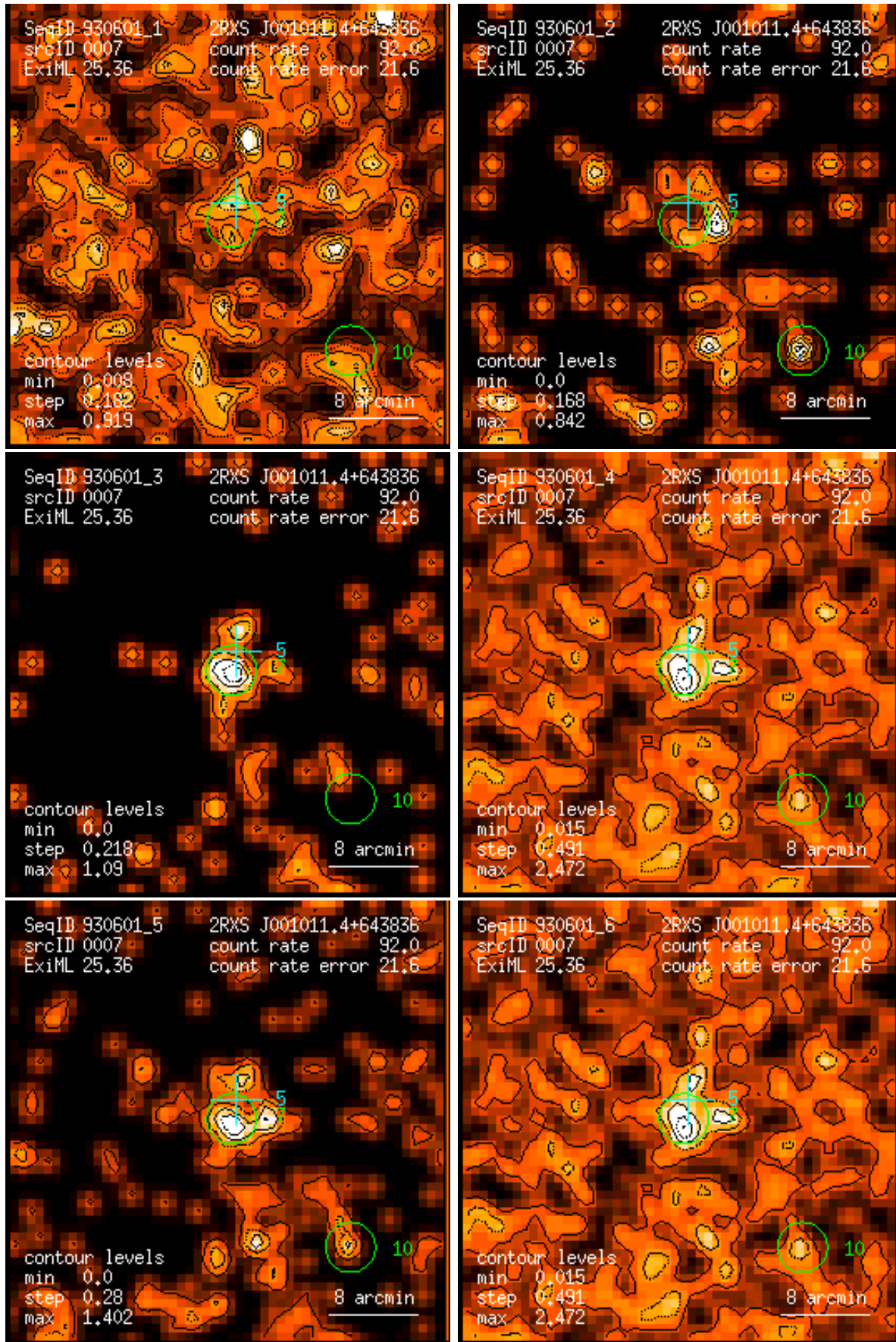
Figure 7: RASS 930601: detection 0007: band rate images, Gaussian filter: (1) PSPC channels 11 – 41, (2) 52 – 90, (3) 91 – 201, (4) 11 – 235, (5) 52 – 201, (6) 11 – 201. Broad band rates in counts/ks. Band rate contour levels in counts/ks/arcmin 2 .
