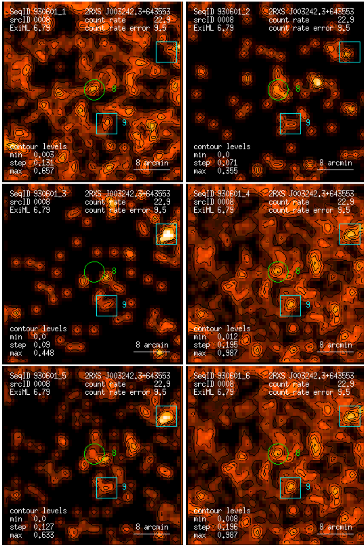
Figure 8: RASS 930601: detection 0008: band rate images, Gaussian filter: (1) PSPC channels 11 – 41, (2) 52 – 90, (3) 91 – 201, (4) 11 – 235, (5) 52 – 201, (6) 11 – 201. Broad band rates in counts/ks. Band rate contour levels in counts/ks/arcmin 2 .
