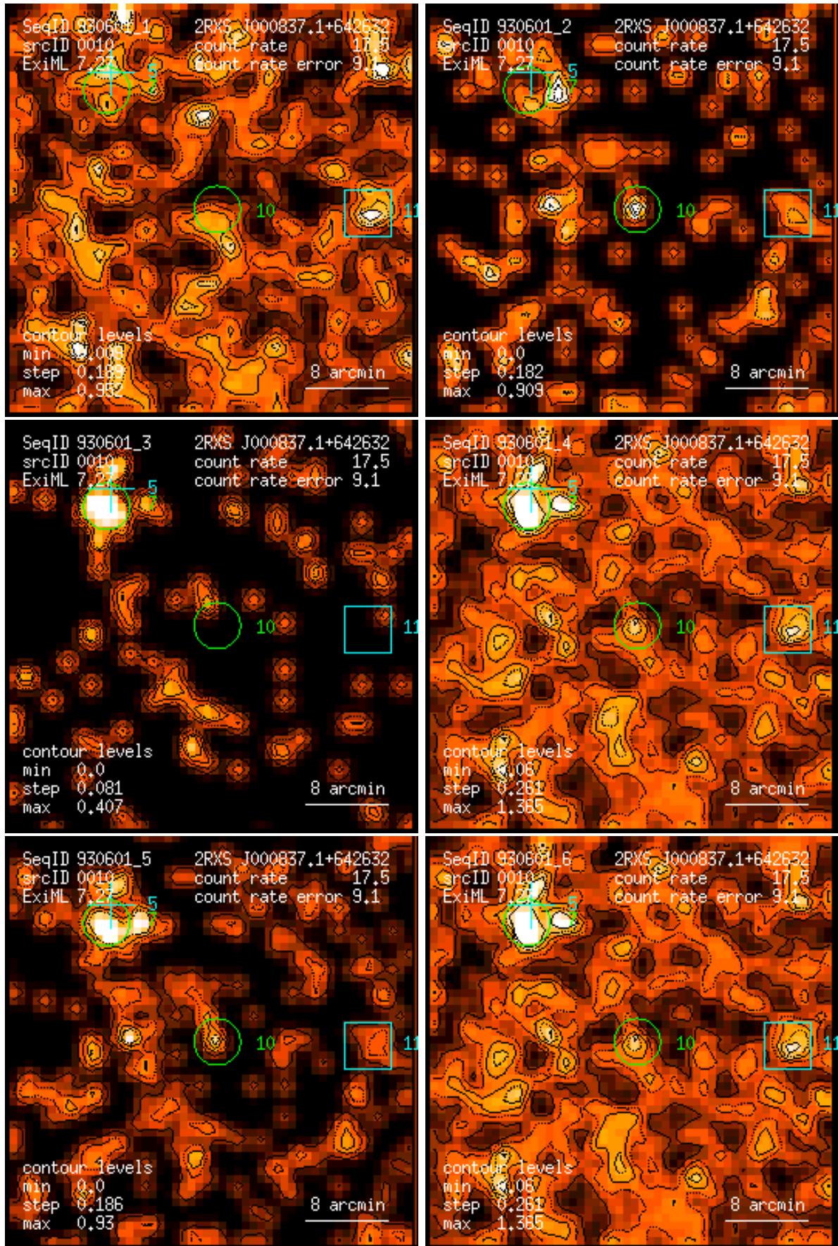
Figure 10: RASS 930601: detection 0010: band rate images, Gaussian filter: (1) PSPC channels 11 – 41, (2) 52 – 90, (3) 91 – 201, (4) 11 – 235, (5) 52 – 201, (6) 11 – 201. Broad band rates in counts/ks. Band rate contour levels in counts/ks/arcmin 2 .
