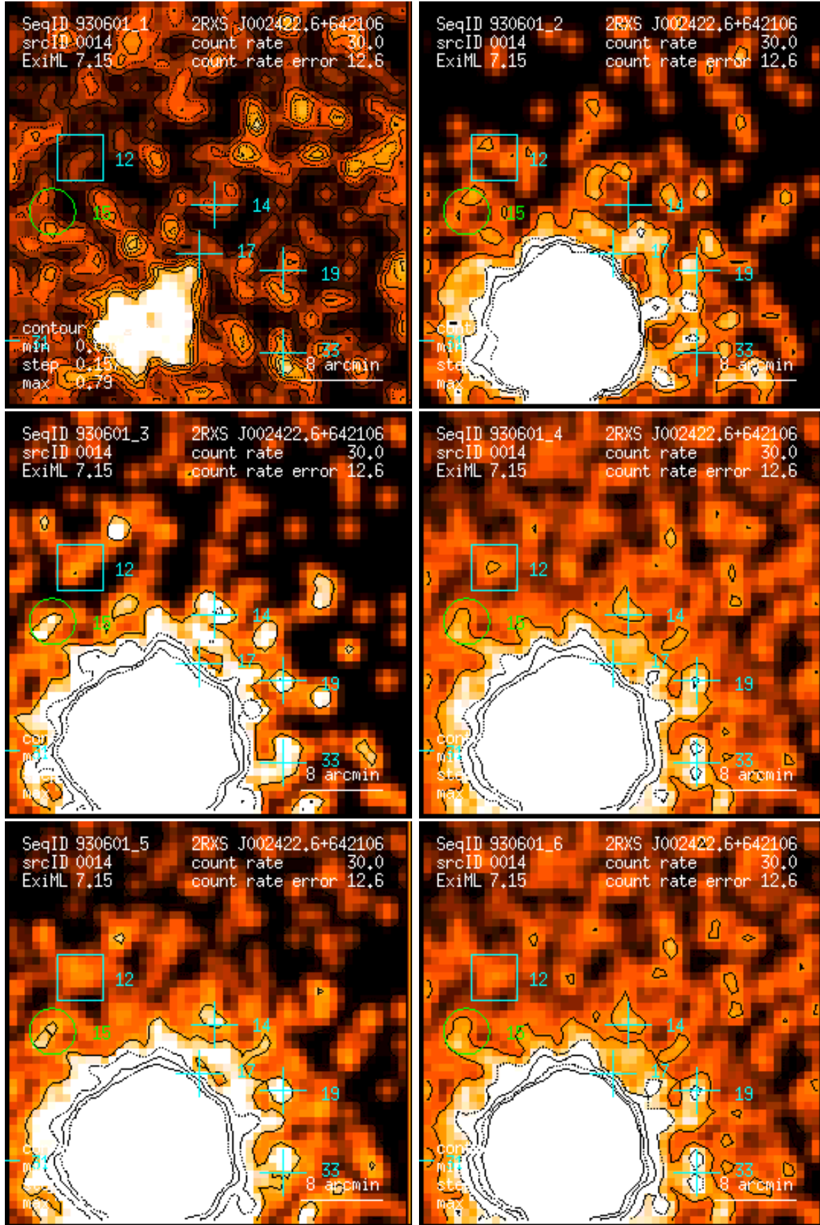
Figure 14: RASS 930601: detection 0014: band rate images, Gaussian filter: (1) PSPC channels 11 – 41, (2) 52 – 90, (3) 91 – 201, (4) 11 – 235, (5) 52 – 201, (6) 11 – 201. Broad band rates in counts/ks. Band rate contour levels in counts/ks/arcmin 2 .
