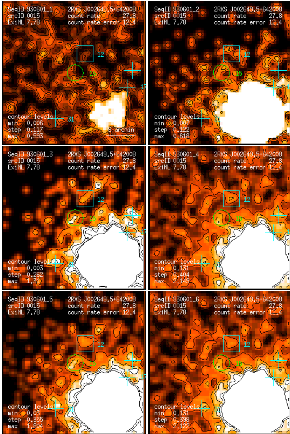
Figure 15: RASS 930601: detection 0015: band rate images, Gaussian filter: (1) PSPC channels 11 – 41, (2) 52 – 90, (3) 91 – 201, (4) 11 – 235, (5) 52 – 201, (6) 11 – 201. Broad band rates in counts/ks. Band rate contour levels in counts/ks/arcmin 2 .
