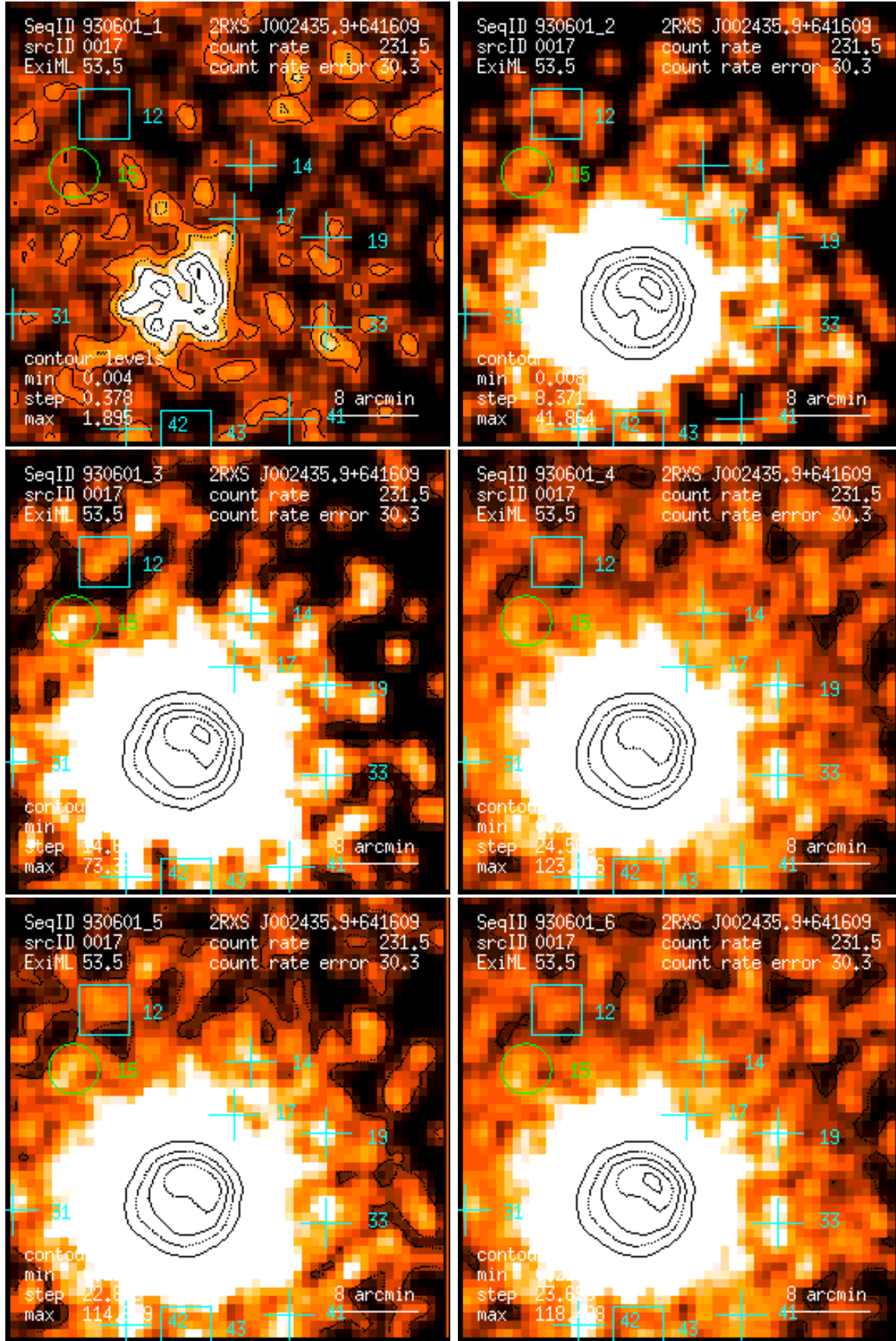
Figure 17: RASS 930601: detection 0017: band rate images, Gaussian filter: (1) PSPC channels 11 – 41, (2) 52 – 90, (3) 91 – 201, (4) 11 – 235, (5) 52 – 201, (6) 11 – 201. Broad band rates in counts/ks. Band rate contour levels in counts/ks/arcmin 2 .
