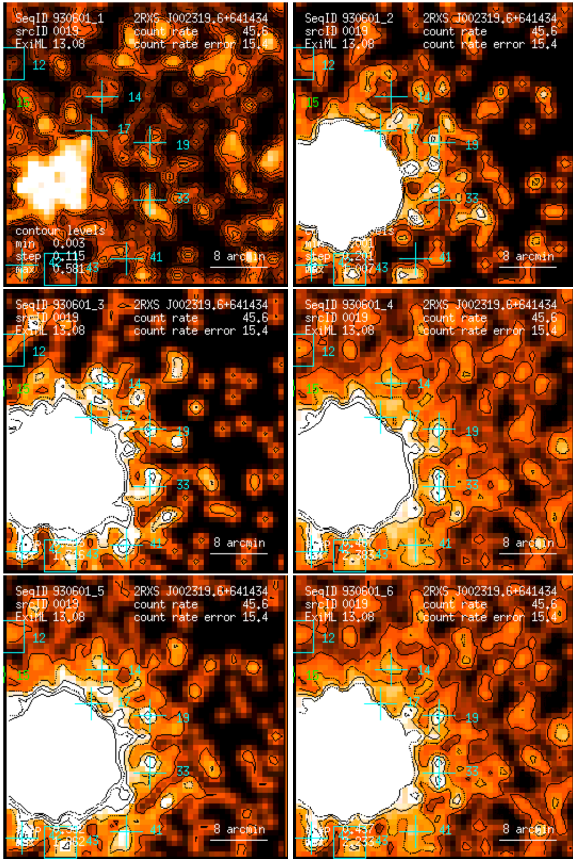
Figure 19: RASS 930601: detection 0019: band rate images, Gaussian filter: (1) PSPC channels 11 – 41, (2) 52 – 90, (3) 91 – 201, (4) 11 – 235, (5) 52 – 201, (6) 11 – 201. Broad band rates in counts/ks. Band rate contour levels in counts/ks/arcmin 2 .
