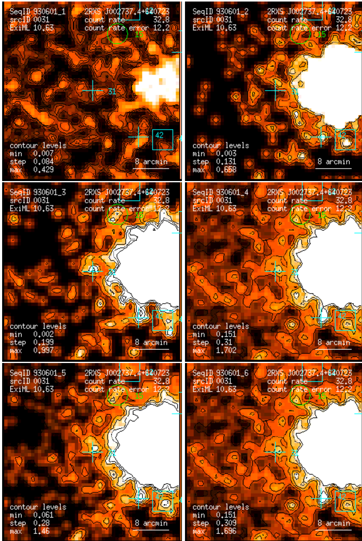
Figure 31: RASS 930601: detection 0031: band rate images, Gaussian filter: (1) PSPC channels 11 – 41, (2) 52 – 90, (3) 91 – 201, (4) 11 – 235, (5) 52 – 201, (6) 11 – 201. Broad band rates in counts/ks. Band rate contour levels in counts/ks/arcmin 2 .
