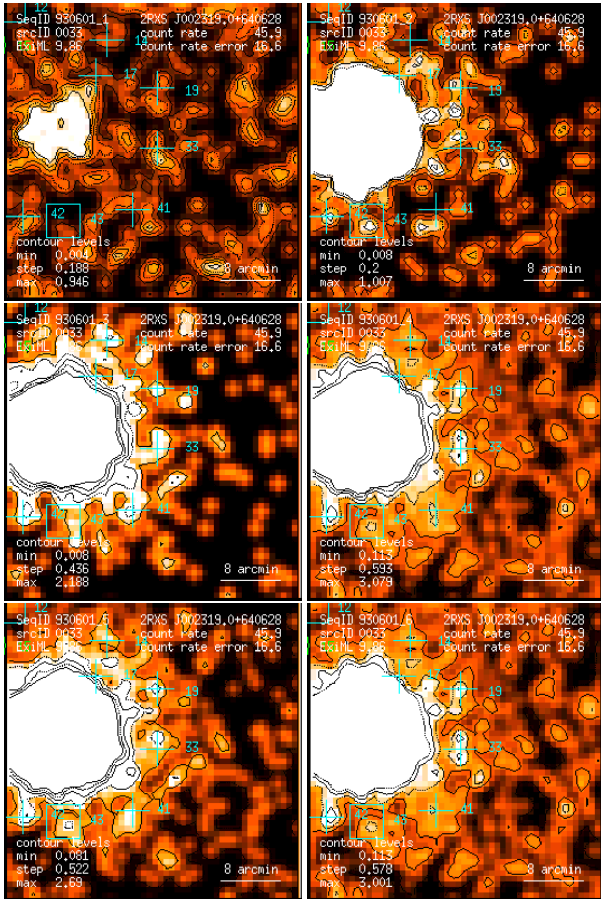
Figure 33: RASS 930601: detection 0033: band rate images, Gaussian filter: (1) PSPC channels 11 – 41, (2) 52 – 90, (3) 91 – 201, (4) 11 – 235, (5) 52 – 201, (6) 11 – 201. Broad band rates in counts/ks. Band rate contour levels in counts/ks/arcmin 2 .
