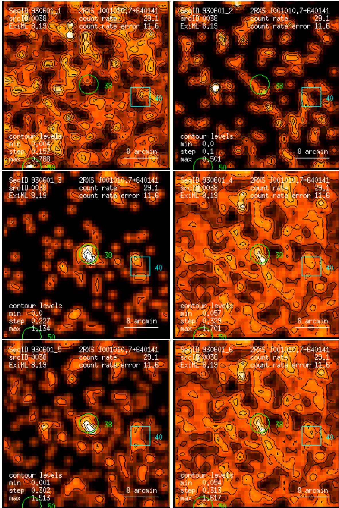
Figure 38: RASS 930601: detection 0038: band rate images, Gaussian filter: (1) PSPC channels 11 – 41, (2) 52 – 90, (3) 91 – 201, (4) 11 – 235, (5) 52 – 201, (6) 11 – 201. Broad band rates in counts/ks. Band rate contour levels in counts/ks/arcmin 2 .
