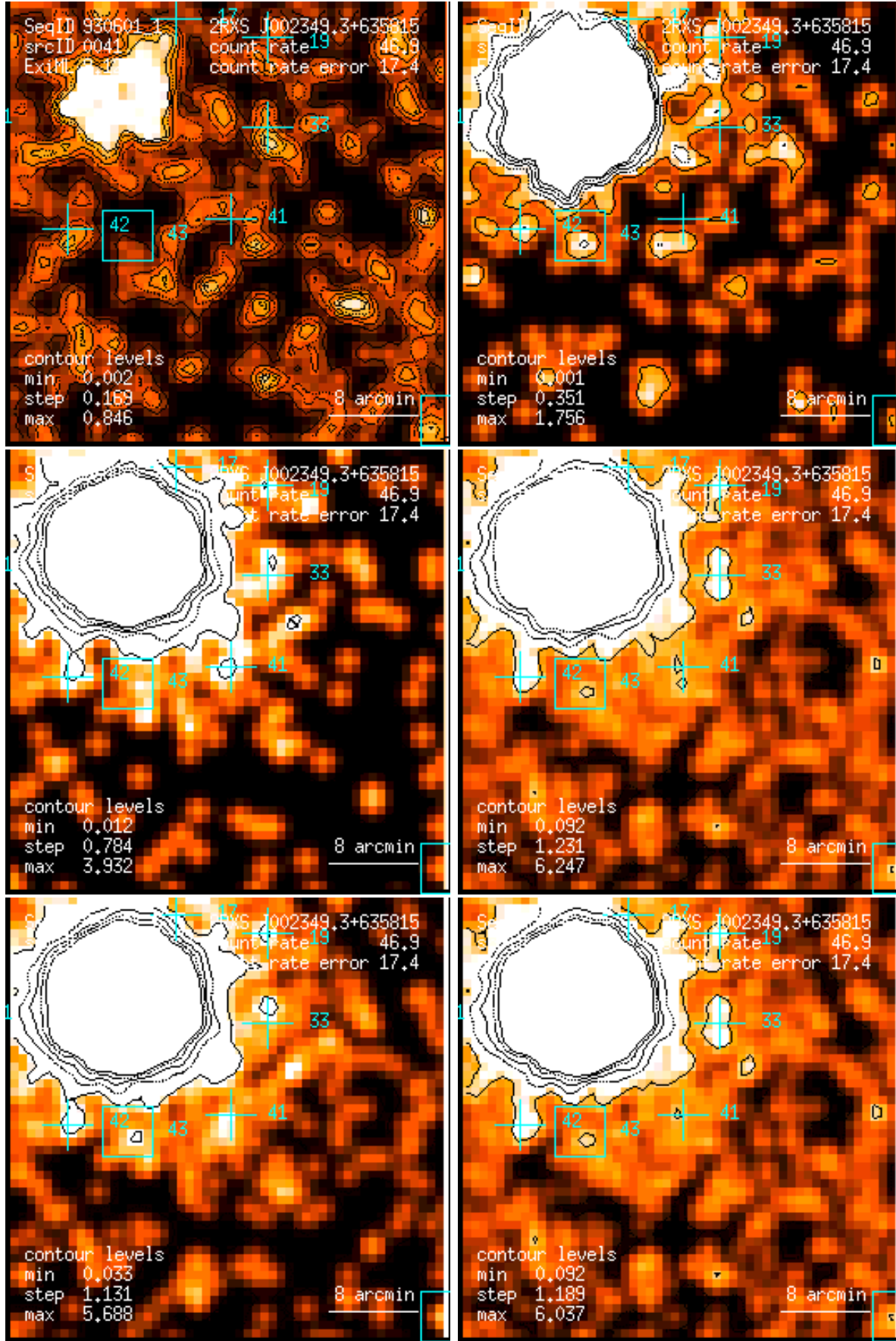
Figure 41: RASS 930601: detection 0041: band rate images, Gaussian filter: (1) PSPC channels 11 – 41, (2) 52 – 90, (3) 91 – 201, (4) 11 – 235, (5) 52 – 201, (6) 11 – 201. Broad band rates in counts/ks. Band rate contour levels in counts/ks/arcmin 2 .
