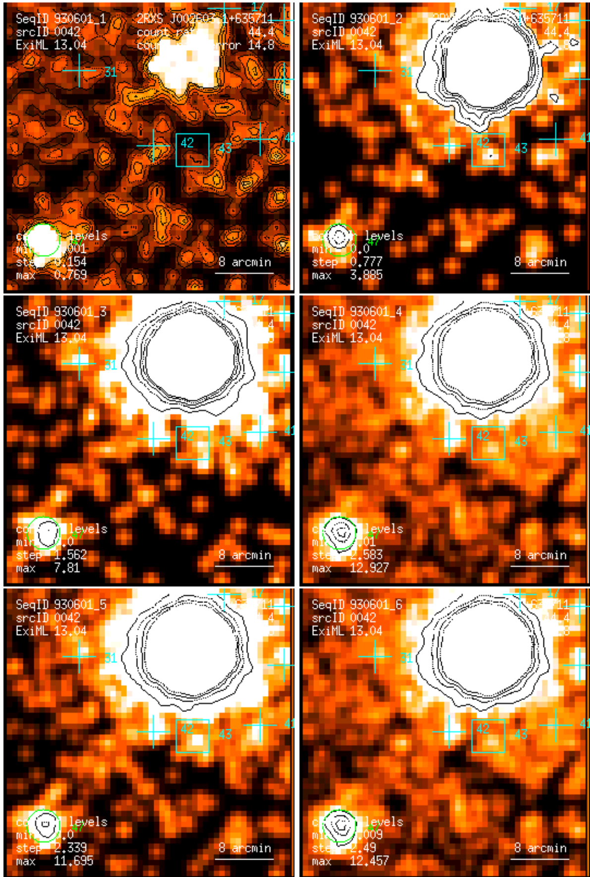
Figure 42: RASS 930601: detection 0042: band rate images, Gaussian filter: (1) PSPC channels 11 – 41, (2) 52 – 90, (3) 91 – 201, (4) 11 – 235, (5) 52 – 201, (6) 11 – 201. Broad band rates in counts/ks. Band rate contour levels in counts/ks/arcmin 2 .
